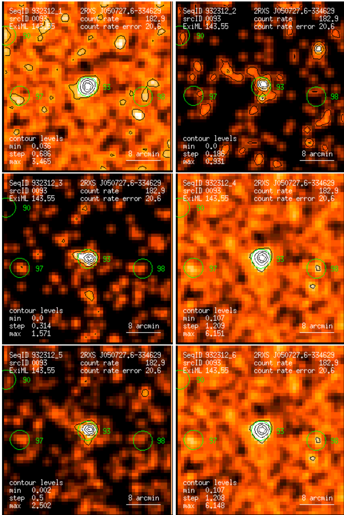
Figure 93: RASS 932312: detection 0093: band rate images, Gaussian filter: (1) PSPC channels 11 – 41, (2) 52 – 90, (3) 91 – 201, (4) 11 – 235, (5) 52 – 201, (6) 11 – 201. Broad band rates in counts/ks. Band rate contour levels in counts/ks/arcmin 2 .
