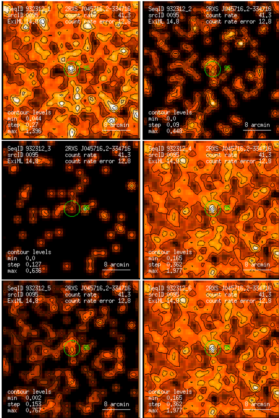
Figure 95: RASS 932312: detection 0095: band rate images, Gaussian filter: (1) PSPC channels 11 – 41, (2) 52 – 90, (3) 91 – 201, (4) 11 – 235, (5) 52 – 201, (6) 11 – 201. Broad band rates in counts/ks. Band rate contour levels in counts/ks/arcmin 2 .
