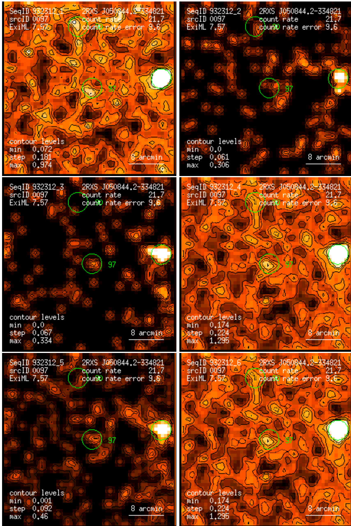
Figure 97: RASS 932312: detection 0097: band rate images, Gaussian filter: (1) PSPC channels 11 – 41, (2) 52 – 90, (3) 91 – 201, (4) 11 – 235, (5) 52 – 201, (6) 11 – 201. Broad band rates in counts/ks. Band rate contour levels in counts/ks/arcmin 2 .
