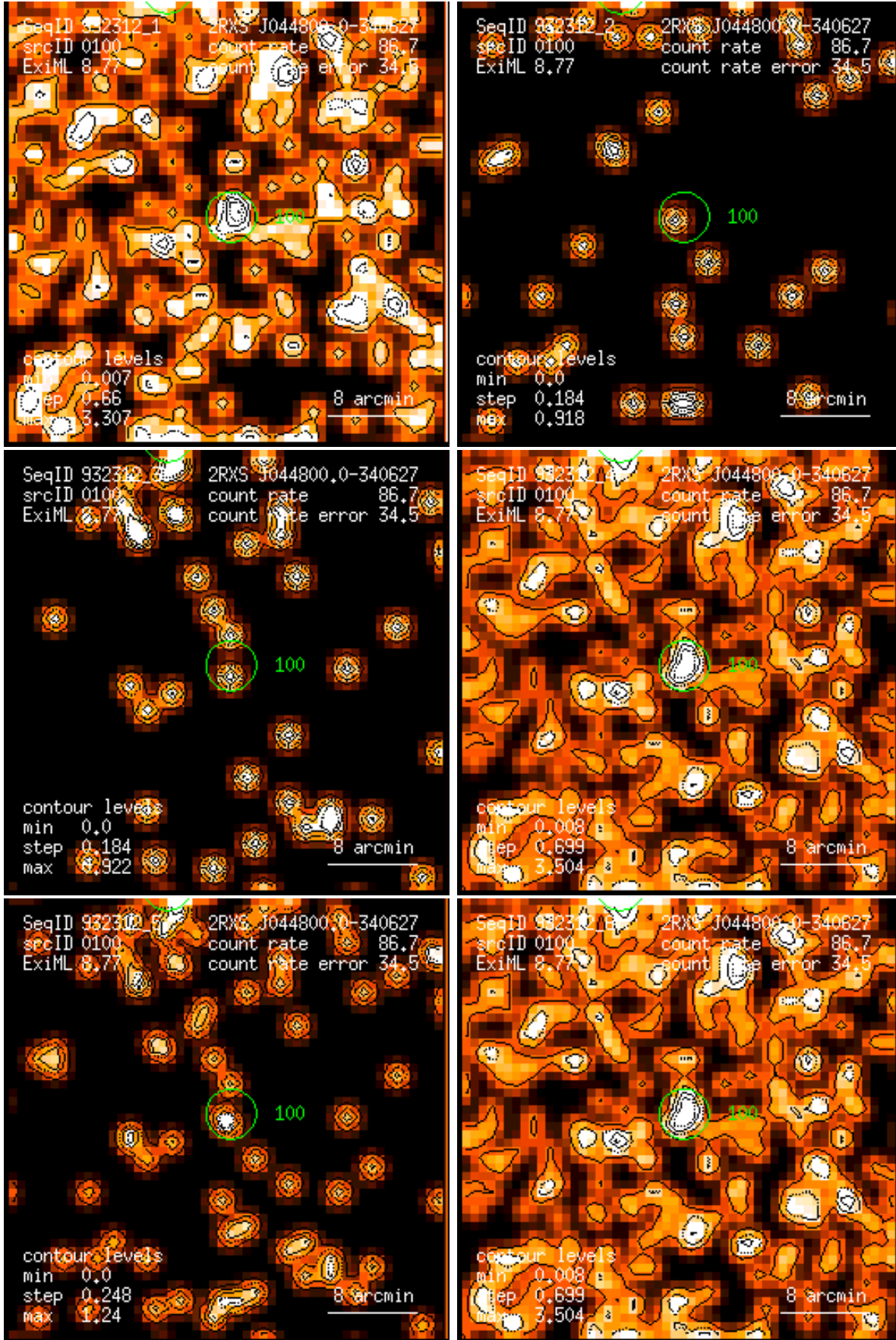
Figure 100: RASS 932312: detection 0100: band rate images, Gaussian filter: (1) PSPC channels 11 – 41, (2) 52 – 90, (3) 91 – 201, (4) 11 – 235, (5) 52 – 201, (6) 11 – 201. Broad band rates in counts/ks. Band rate contour levels in counts/ks/arcmin 2 .
