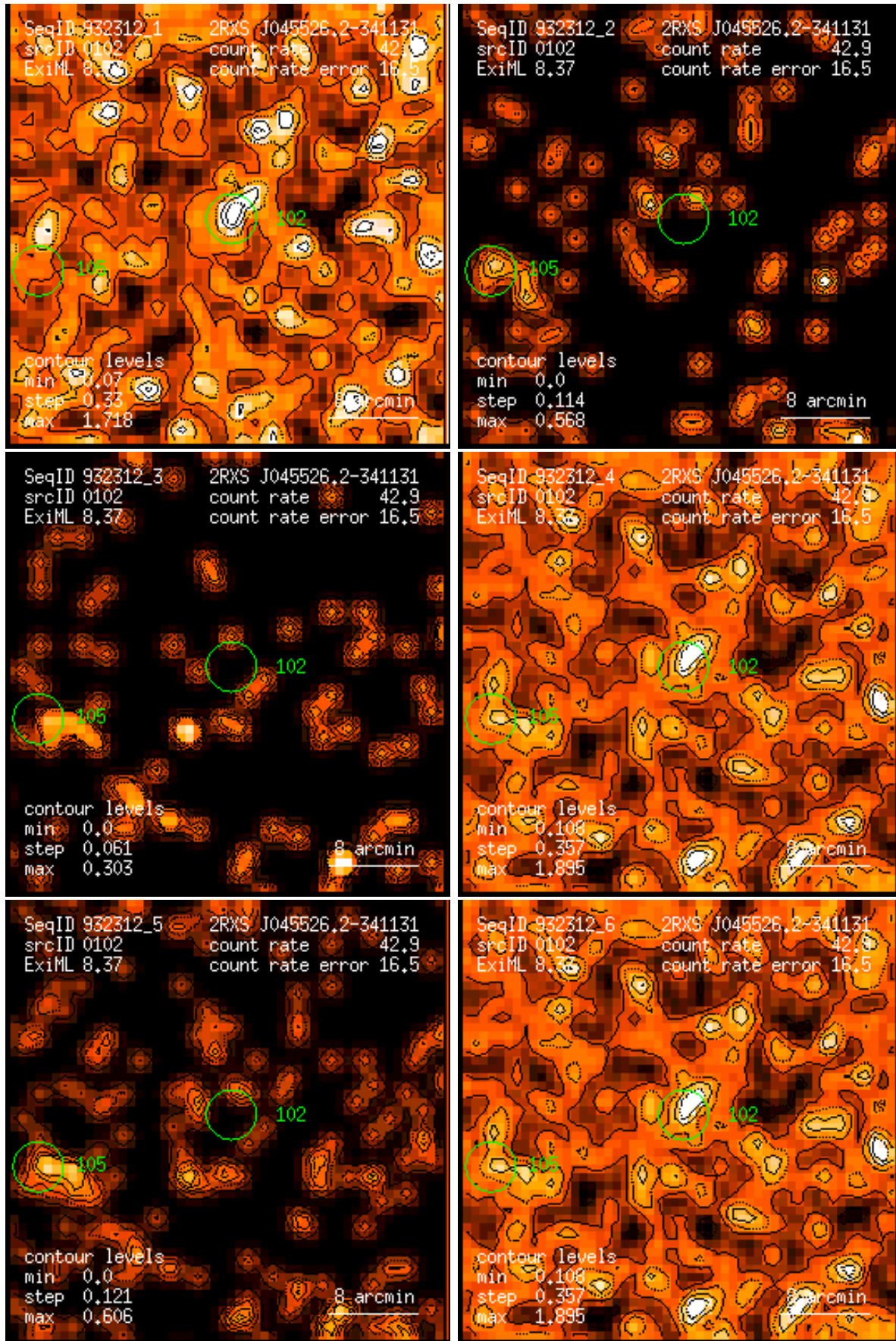
Figure 102: RASS 932312: detection 0102: band rate images, Gaussian filter: (1) PSPC channels 11 – 41, (2) 52 – 90, (3) 91 – 201, (4) 11 – 235, (5) 52 – 201, (6) 11 – 201. Broad band rates in counts/ks. Band rate contour levels in counts/ks/arcmin 2 .
