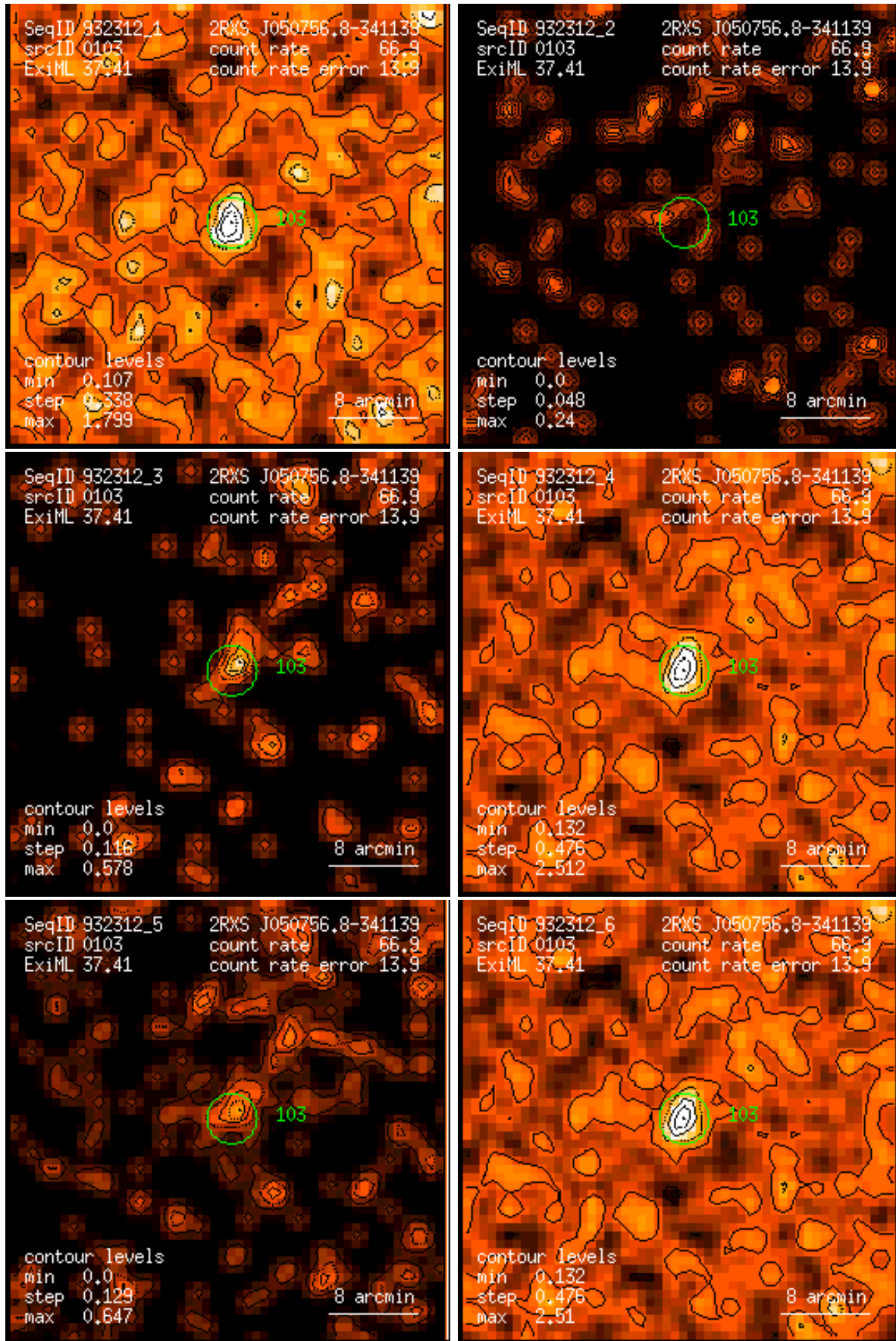
Figure 103: RASS 932312: detection 0103: band rate images, Gaussian filter: (1) PSPC channels 11 – 41, (2) 52 – 90, (3) 91 – 201, (4) 11 – 235, (5) 52 – 201, (6) 11 – 201. Broad band rates in counts/ks. Band rate contour levels in counts/ks/arcmin 2 .
