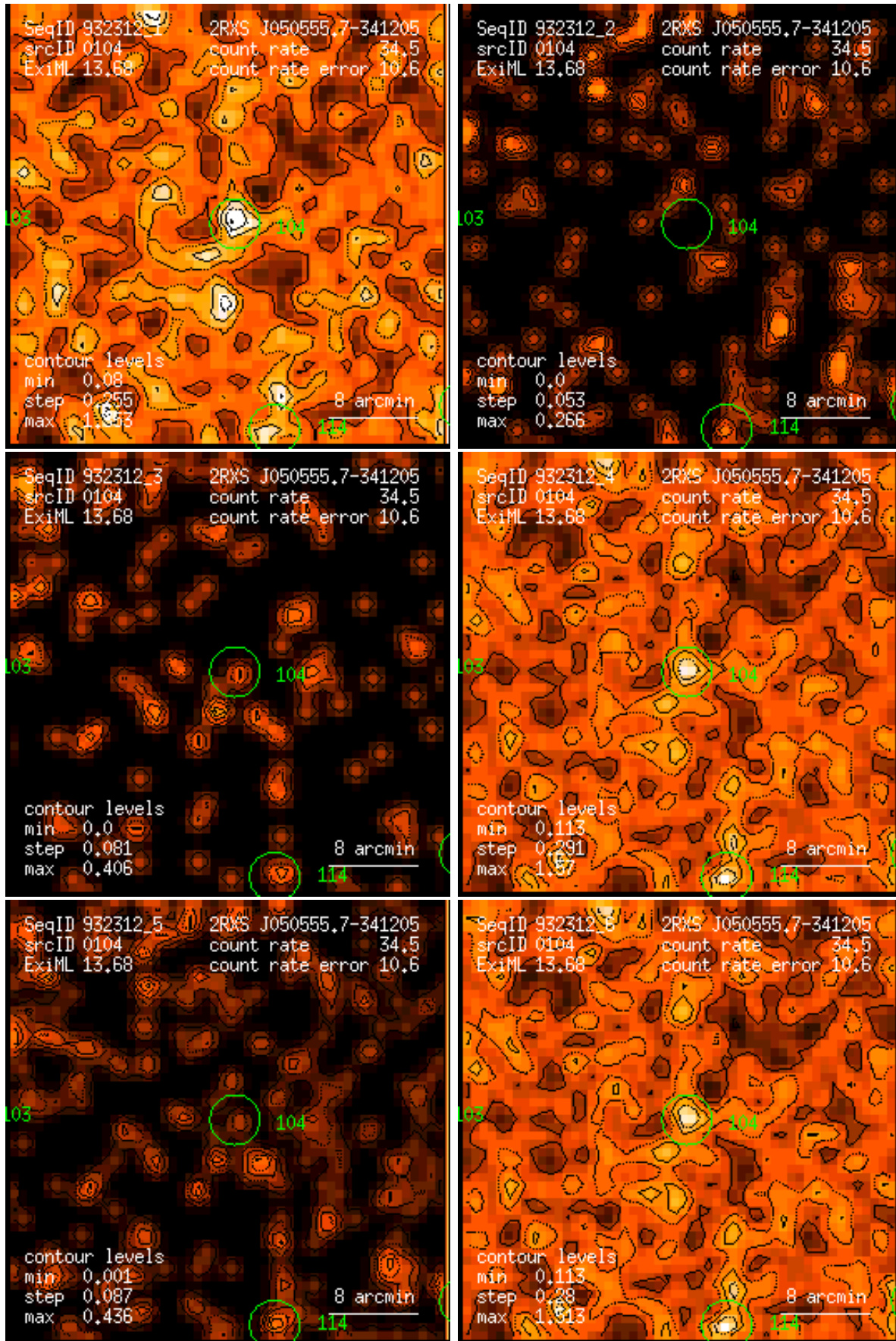
Figure 104: RASS 932312: detection 0104: band rate images, Gaussian filter: (1) PSPC channels 11 – 41, (2) 52 – 90, (3) 91 – 201, (4) 11 – 235, (5) 52 – 201, (6) 11 – 201. Broad band rates in counts/ks. Band rate contour levels in counts/ks/arcmin 2 .
