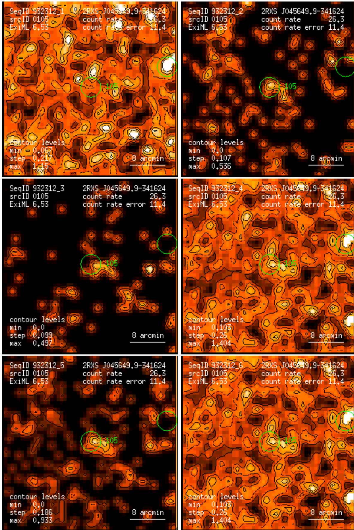
Figure 105: RASS 932312: detection 0105: band rate images, Gaussian filter: (1) PSPC channels 11 – 41, (2) 52 – 90, (3) 91 – 201, (4) 11 – 235, (5) 52 – 201, (6) 11 – 201. Broad band rates in counts/ks. Band rate contour levels in counts/ks/arcmin 2 .
