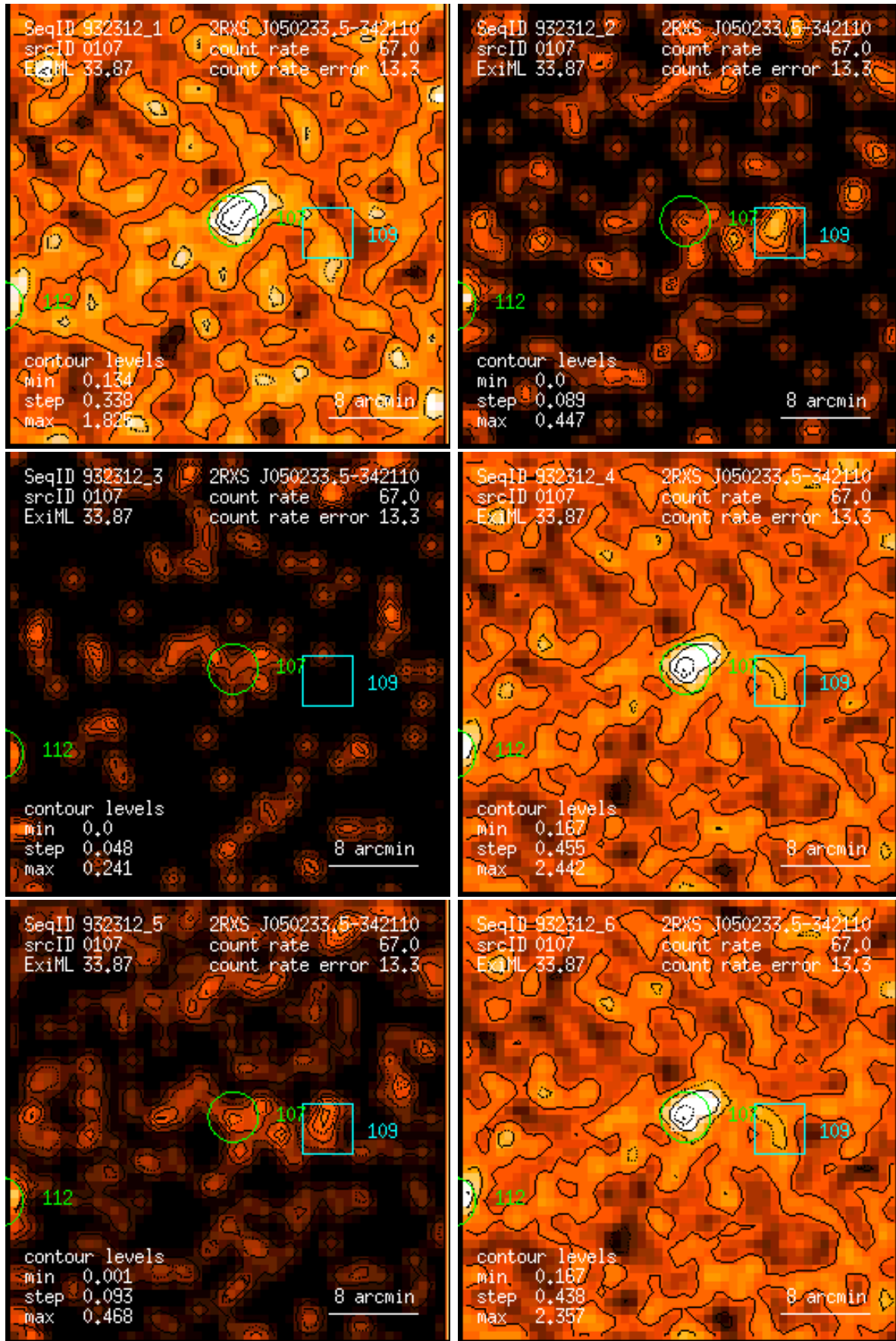
Figure 107: RASS 932312: detection 0107: band rate images, Gaussian filter: (1) PSPC channels 11 – 41, (2) 52 – 90, (3) 91 – 201, (4) 11 – 235, (5) 52 – 201, (6) 11 – 201. Broad band rates in counts/ks. Band rate contour levels in counts/ks/arcmin 2 .
