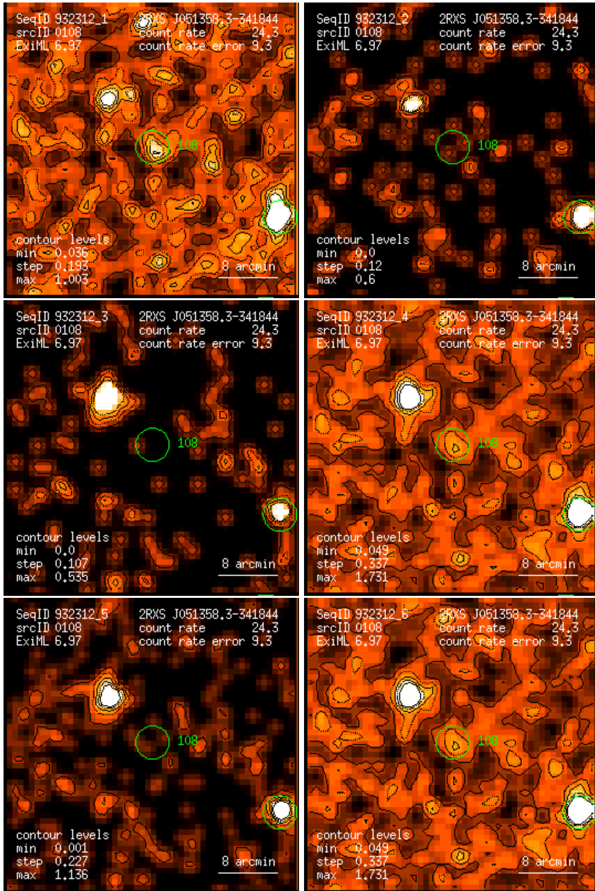
Figure 108: RASS 932312: detection 0108: band rate images, Gaussian filter: (1) PSPC channels 11 – 41, (2) 52 – 90, (3) 91 – 201, (4) 11 – 235, (5) 52 – 201, (6) 11 – 201. Broad band rates in counts/ks. Band rate contour levels in counts/ks/arcmin 2 .
