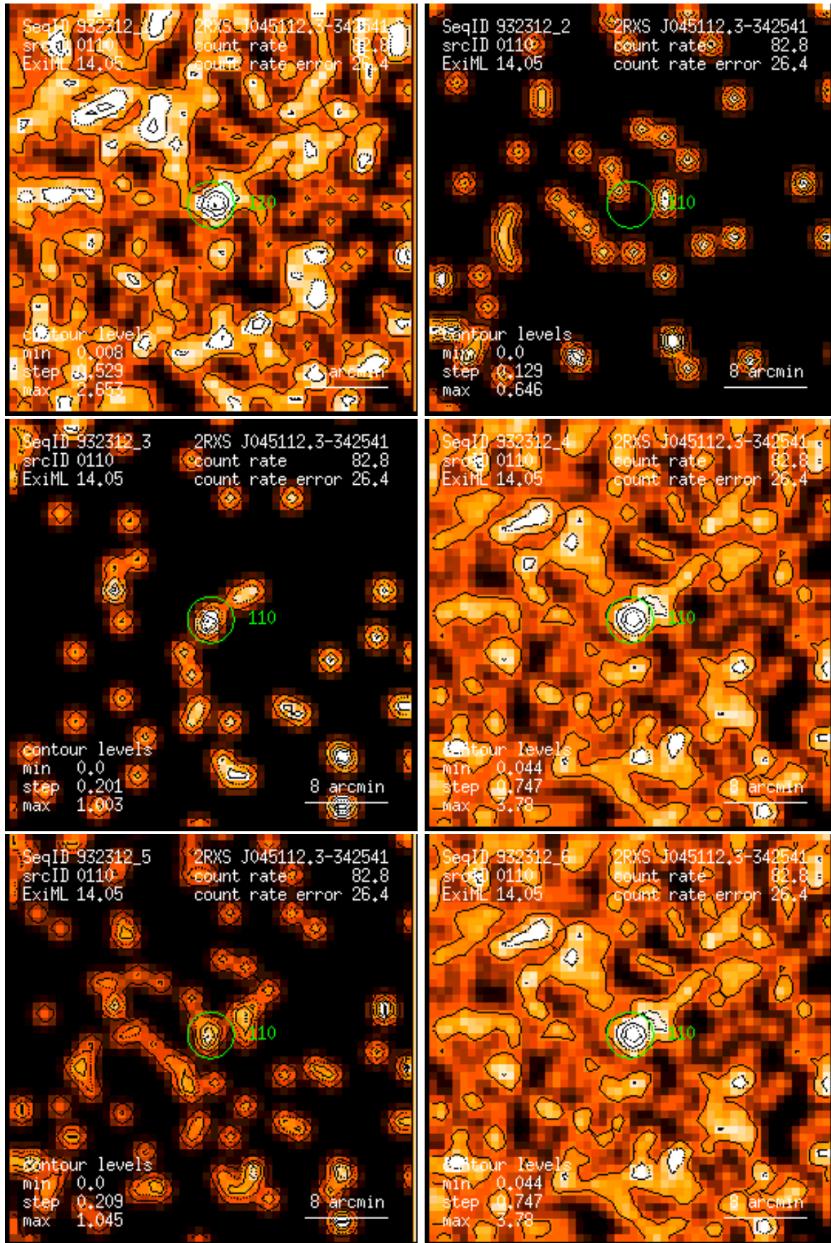
Figure 110: RASS 932312: detection 0110: band rate images, Gaussian filter: (1) PSPC channels 11 – 41, (2) 52 – 90, (3) 91 – 201, (4) 11 – 235, (5) 52 – 201, (6) 11 – 201. Broad band rates in counts/ks. Band rate contour levels in counts/ks/arcmin 2 .
