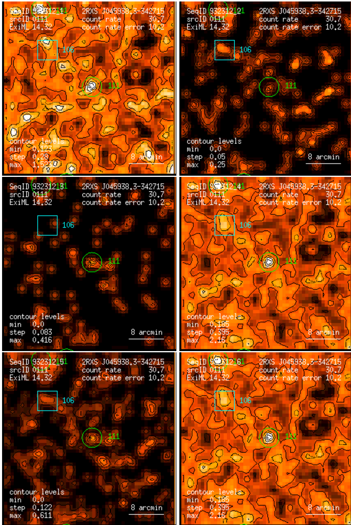
Figure 111: RASS 932312: detection 0111: band rate images, Gaussian filter: (1) PSPC channels 11 – 41, (2) 52 – 90, (3) 91 – 201, (4) 11 – 235, (5) 52 – 201, (6) 11 – 201. Broad band rates in counts/ks. Band rate contour levels in counts/ks/arcmin 2 .
