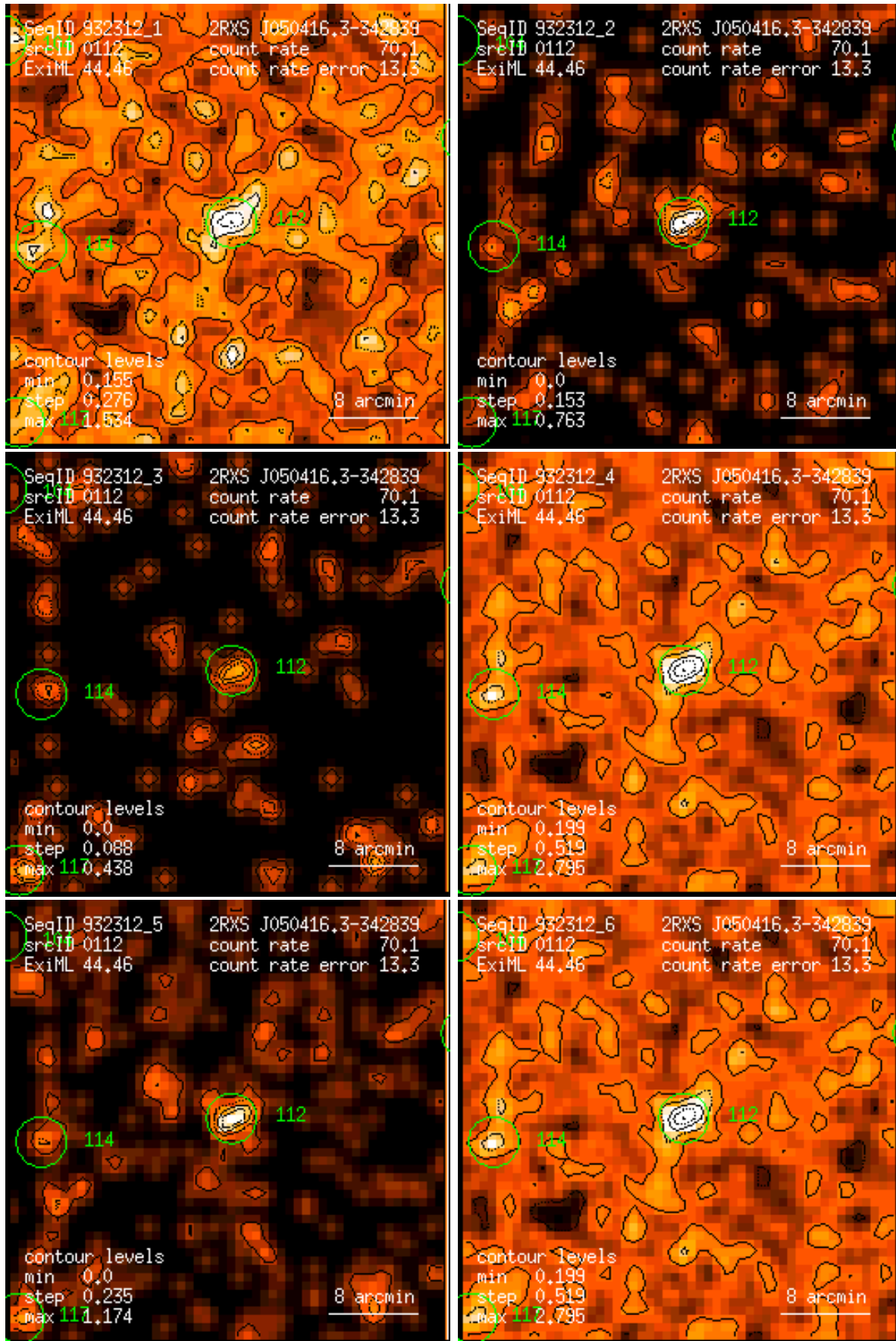
Figure 112: RASS 932312: detection 0112: band rate images, Gaussian filter: (1) PSPC channels 11 – 41, (2) 52 – 90, (3) 91 – 201, (4) 11 – 235, (5) 52 – 201, (6) 11 – 201. Broad band rates in counts/ks. Band rate contour levels in counts/ks/arcmin 2 .
