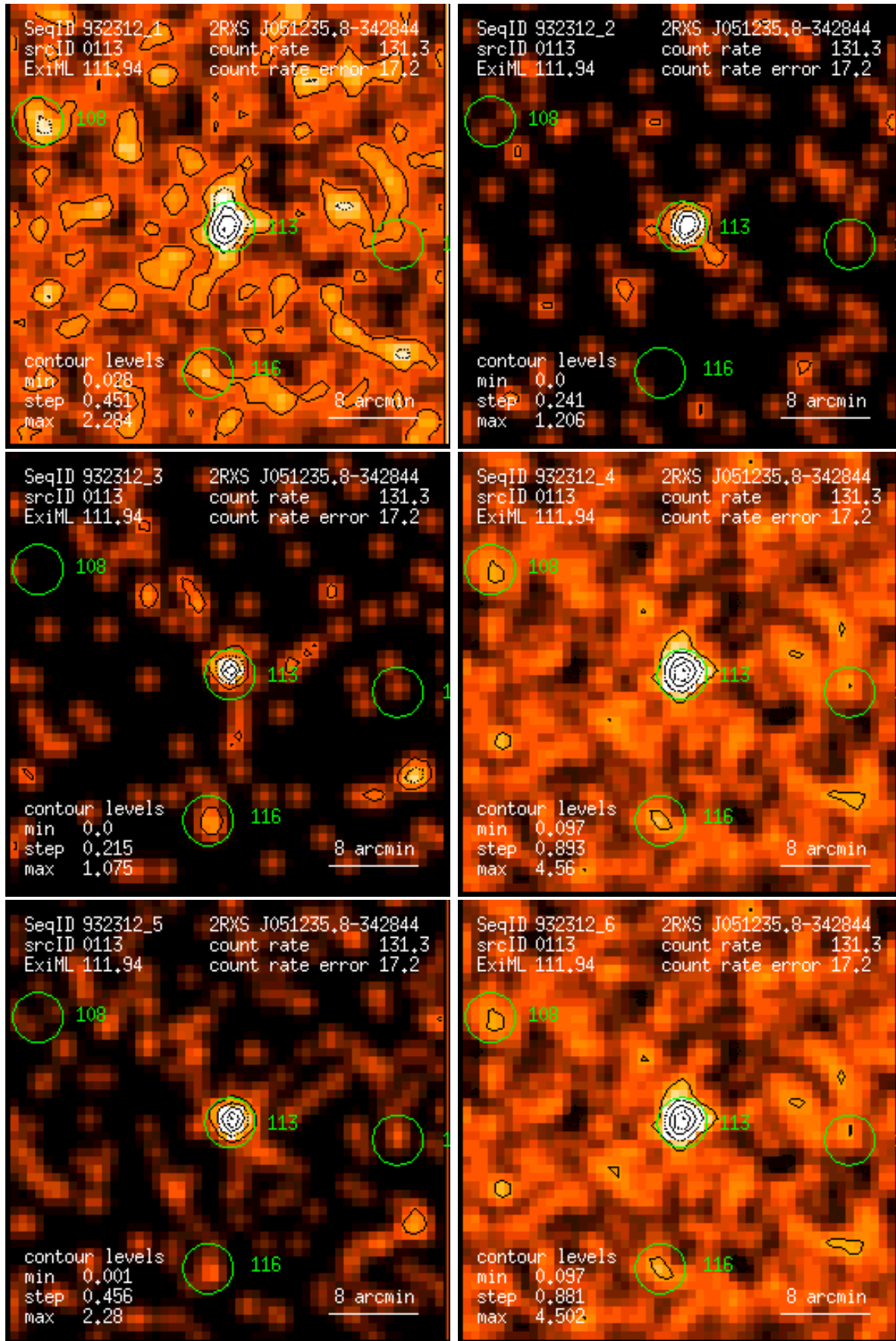
Figure 113: RASS 932312: detection 0113: band rate images, Gaussian filter: (1) PSPC channels 11 – 41, (2) 52 – 90, (3) 91 – 201, (4) 11 – 235, (5) 52 – 201, (6) 11 – 201. Broad band rates in counts/ks. Band rate contour levels in counts/ks/arcmin 2 .
