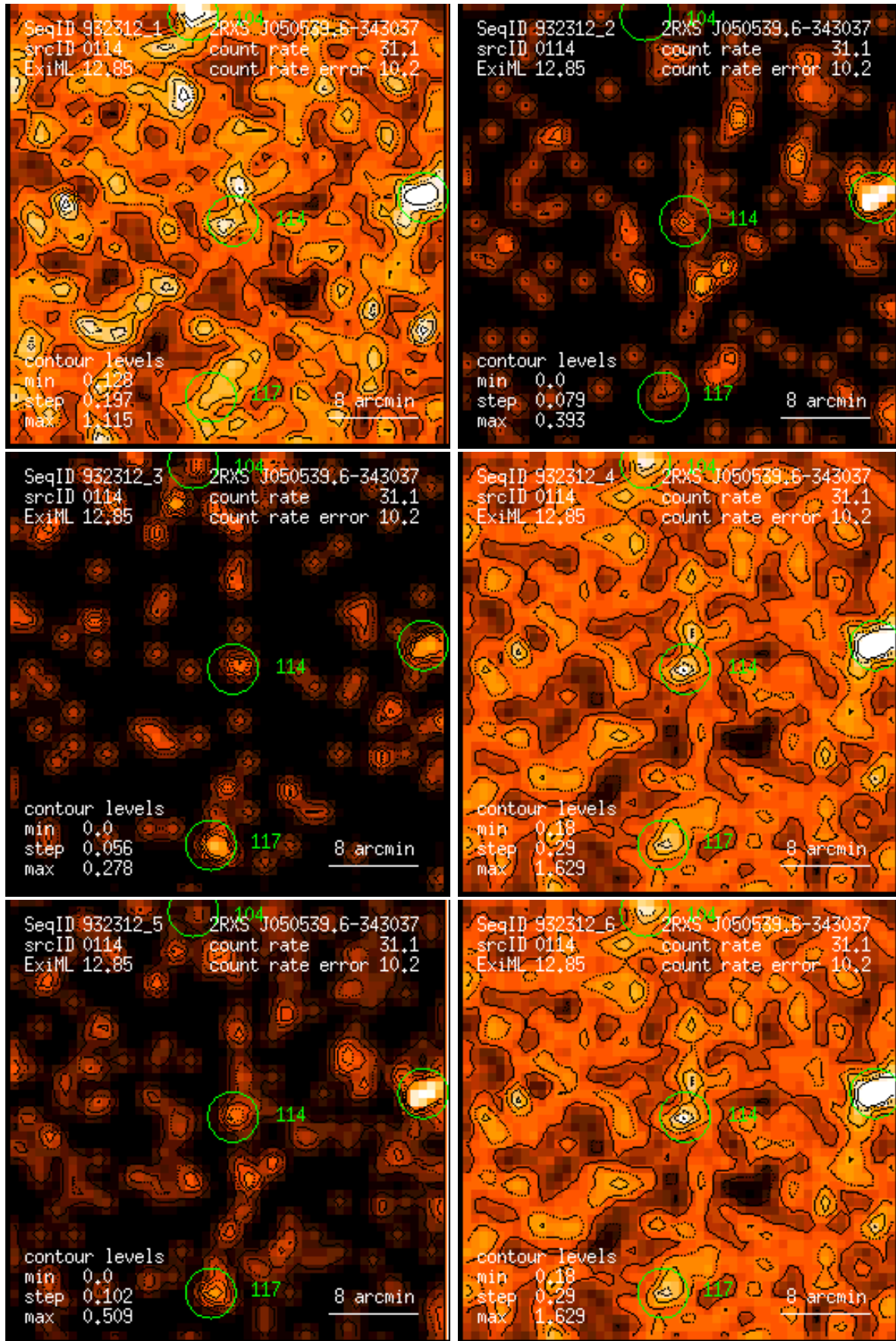
Figure 114: RASS 932312: detection 0114: band rate images, Gaussian filter: (1) PSPC channels 11 – 41, (2) 52 – 90, (3) 91 – 201, (4) 11 – 235, (5) 52 – 201, (6) 11 – 201. Broad band rates in counts/ks. Band rate contour levels in counts/ks/arcmin 2 .
