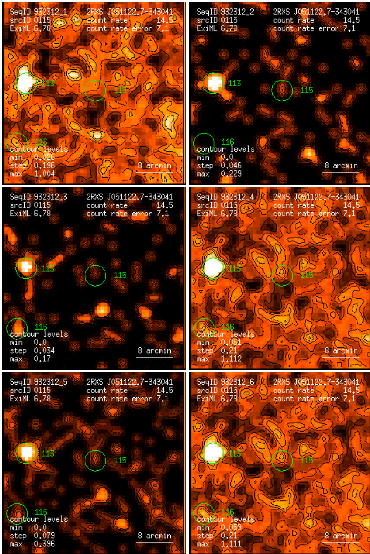
Figure 115: RASS 932312: detection 0115: band rate images, Gaussian filter: (1) PSPC channels 11 – 41, (2) 52 – 90, (3) 91 – 201, (4) 11 – 235, (5) 52 – 201, (6) 11 – 201. Broad band rates in counts/ks. Band rate contour levels in counts/ks/arcmin 2 .
