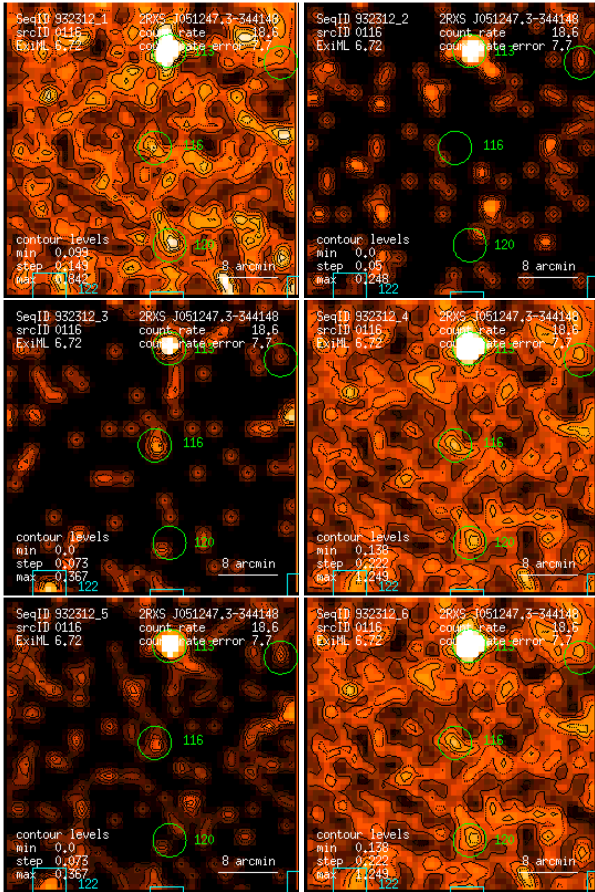
Figure 116: RASS 932312: detection 0116: band rate images, Gaussian filter: (1) PSPC channels 11 – 41, (2) 52 – 90, (3) 91 – 201, (4) 11 – 235, (5) 52 – 201, (6) 11 – 201. Broad band rates in counts/ks. Band rate contour levels in counts/ks/arcmin 2 .
