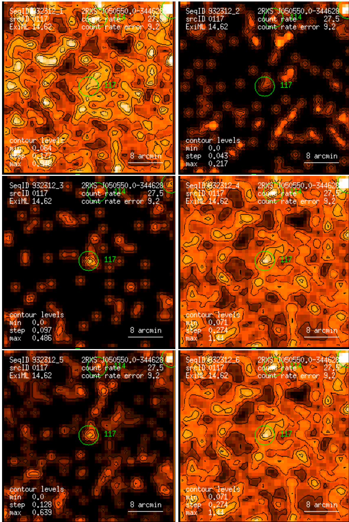
Figure 117: RASS 932312: detection 0117: band rate images, Gaussian filter: (1) PSPC channels 11 – 41, (2) 52 – 90, (3) 91 – 201, (4) 11 – 235, (5) 52 – 201, (6) 11 – 201. Broad band rates in counts/ks. Band rate contour levels in counts/ks/arcmin 2 .
