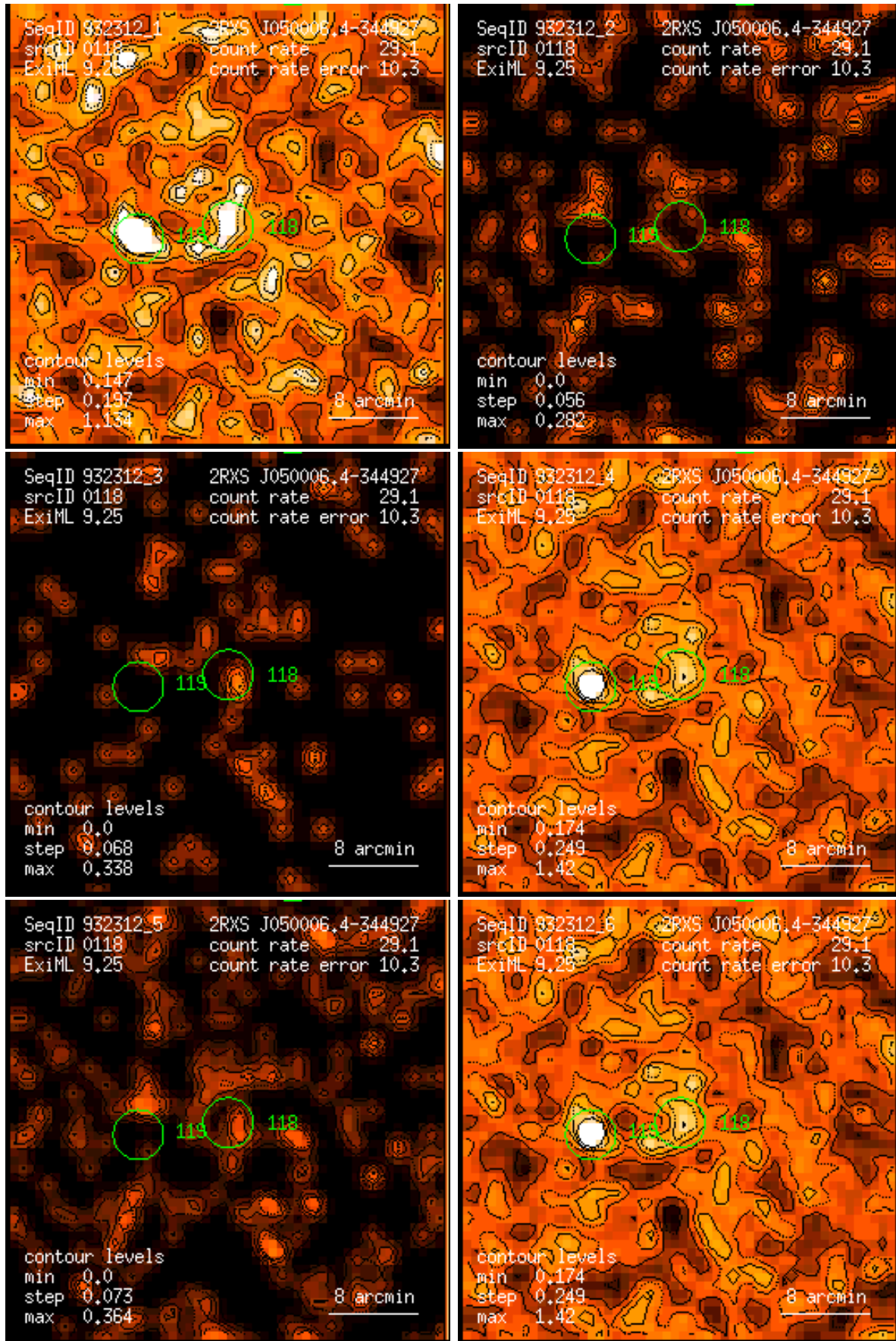
Figure 118: RASS 932312: detection 0118: band rate images, Gaussian filter: (1) PSPC channels 11 – 41, (2) 52 – 90, (3) 91 – 201, (4) 11 – 235, (5) 52 – 201, (6) 11 – 201. Broad band rates in counts/ks. Band rate contour levels in counts/ks/arcmin 2 .
