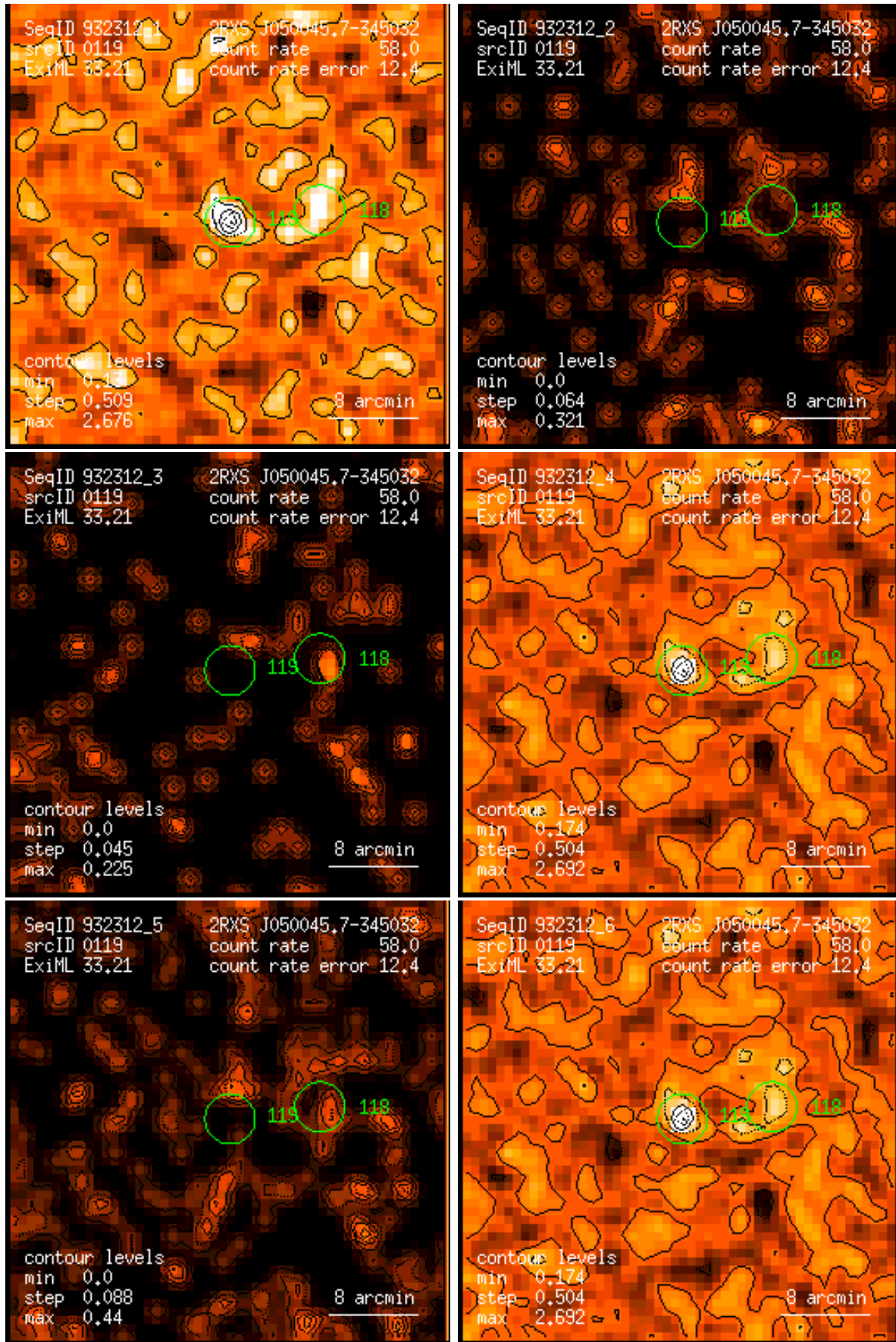
Figure 119: RASS 932312: detection 0119: band rate images, Gaussian filter: (1) PSPC channels 11 – 41, (2) 52 – 90, (3) 91 – 201, (4) 11 – 235, (5) 52 – 201, (6) 11 – 201. Broad band rates in counts/ks. Band rate contour levels in counts/ks/arcmin 2 .
