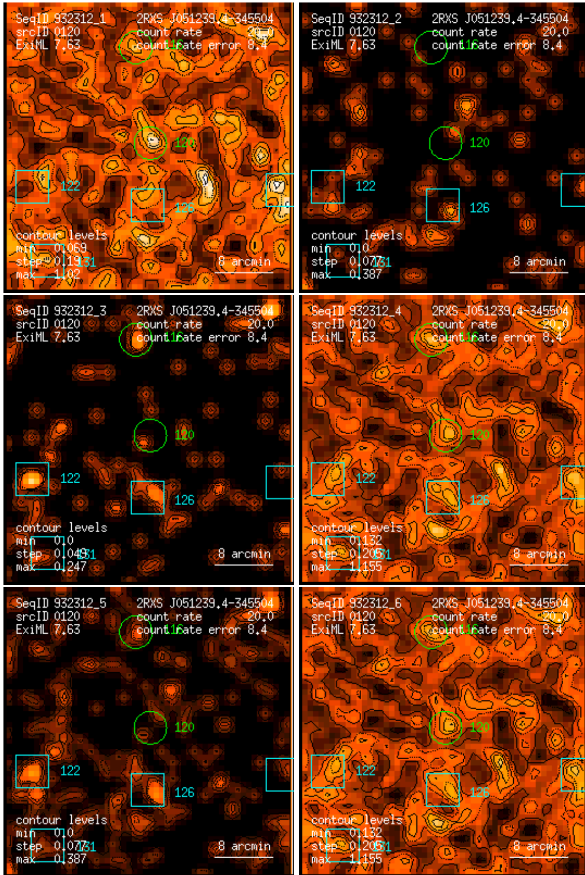
Figure 120: RASS 932312: detection 0120: band rate images, Gaussian filter: (1) PSPC channels 11 – 41, (2) 52 – 90, (3) 91 – 201, (4) 11 – 235, (5) 52 – 201, (6) 11 – 201. Broad band rates in counts/ks. Band rate contour levels in counts/ks/arcmin 2 .
