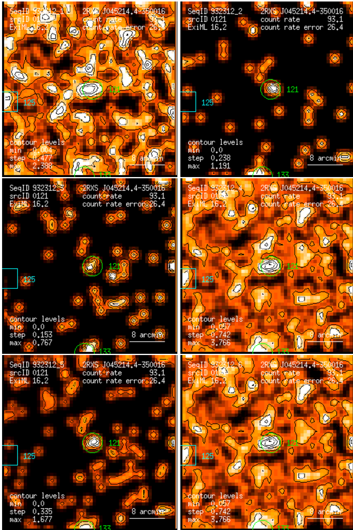
Figure 121: RASS 932312: detection 0121: band rate images, Gaussian filter: (1) PSPC channels 11 – 41, (2) 52 – 90, (3) 91 – 201, (4) 11 – 235, (5) 52 – 201, (6) 11 – 201. Broad band rates in counts/ks. Band rate contour levels in counts/ks/arcmin 2 .
