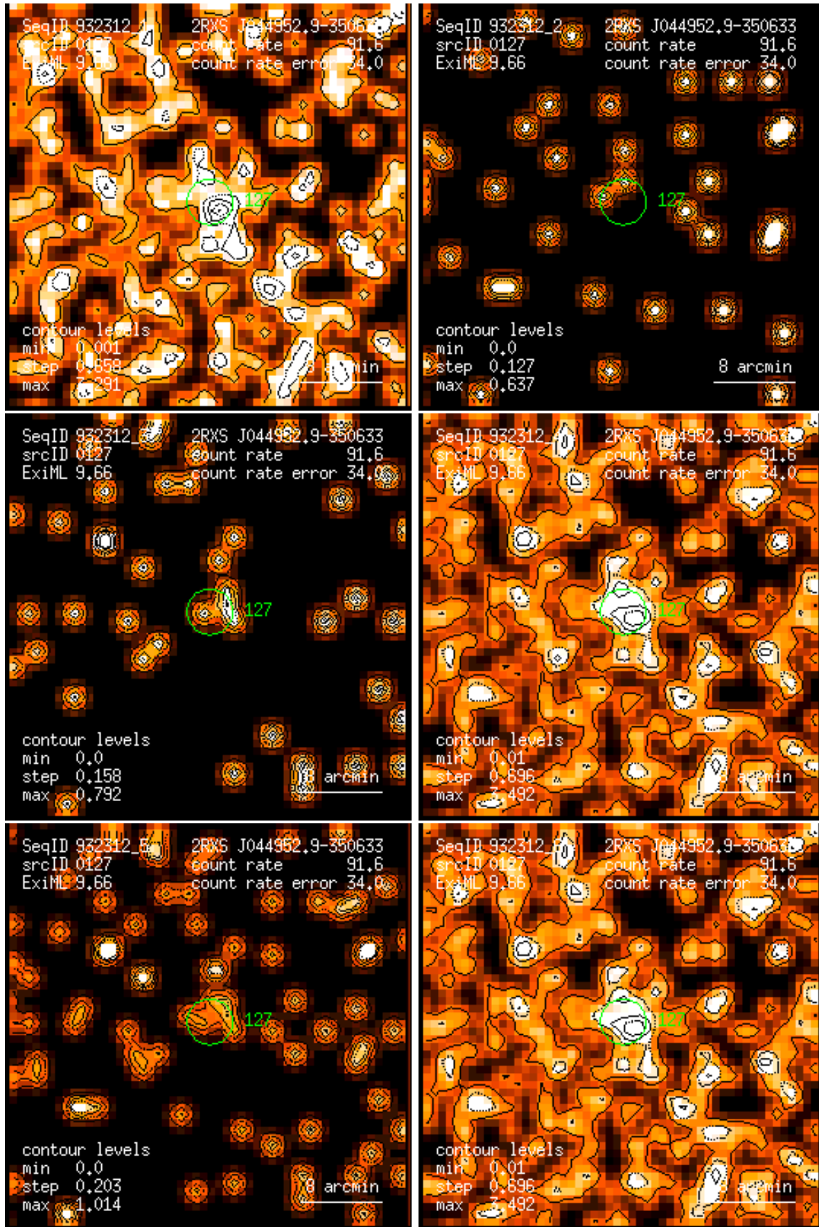
Figure 127: RASS 932312: detection 0127: band rate images, Gaussian filter: (1) PSPC channels 11 – 41, (2) 52 – 90, (3) 91 – 201, (4) 11 – 235, (5) 52 – 201, (6) 11 – 201. Broad band rates in counts/ks. Band rate contour levels in counts/ks/arcmin 2 .
