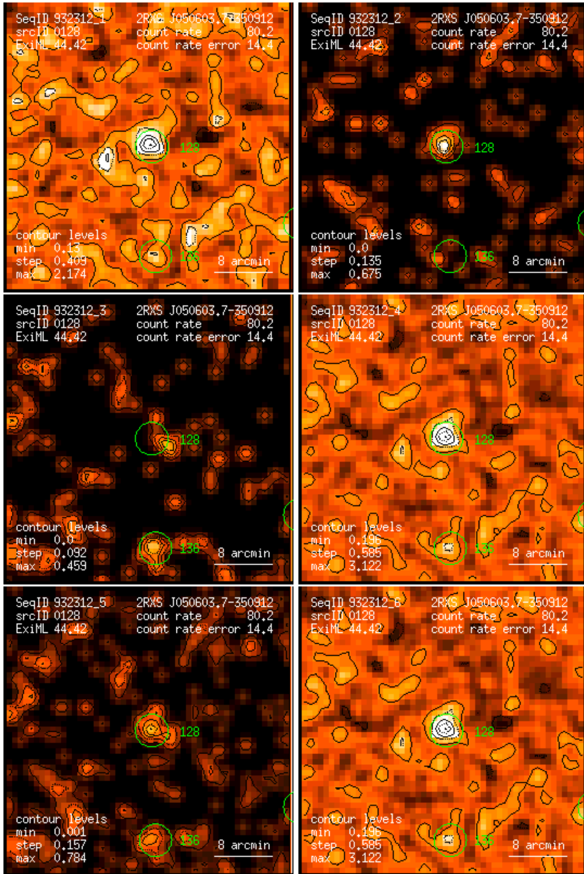
Figure 128: RASS 932312: detection 0128: band rate images, Gaussian filter: (1) PSPC channels 11 – 41, (2) 52 – 90, (3) 91 – 201, (4) 11 – 235, (5) 52 – 201, (6) 11 – 201. Broad band rates in counts/ks. Band rate contour levels in counts/ks/arcmin 2 .
