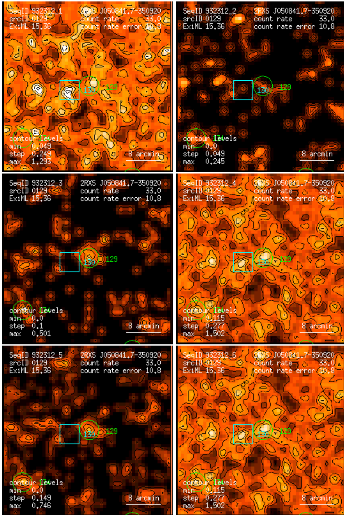
Figure 129: RASS 932312: detection 0129: band rate images, Gaussian filter: (1) PSPC channels 11 – 41, (2) 52 – 90, (3) 91 – 201, (4) 11 – 235, (5) 52 – 201, (6) 11 – 201. Broad band rates in counts/ks. Band rate contour levels in counts/ks/arcmin 2 .
