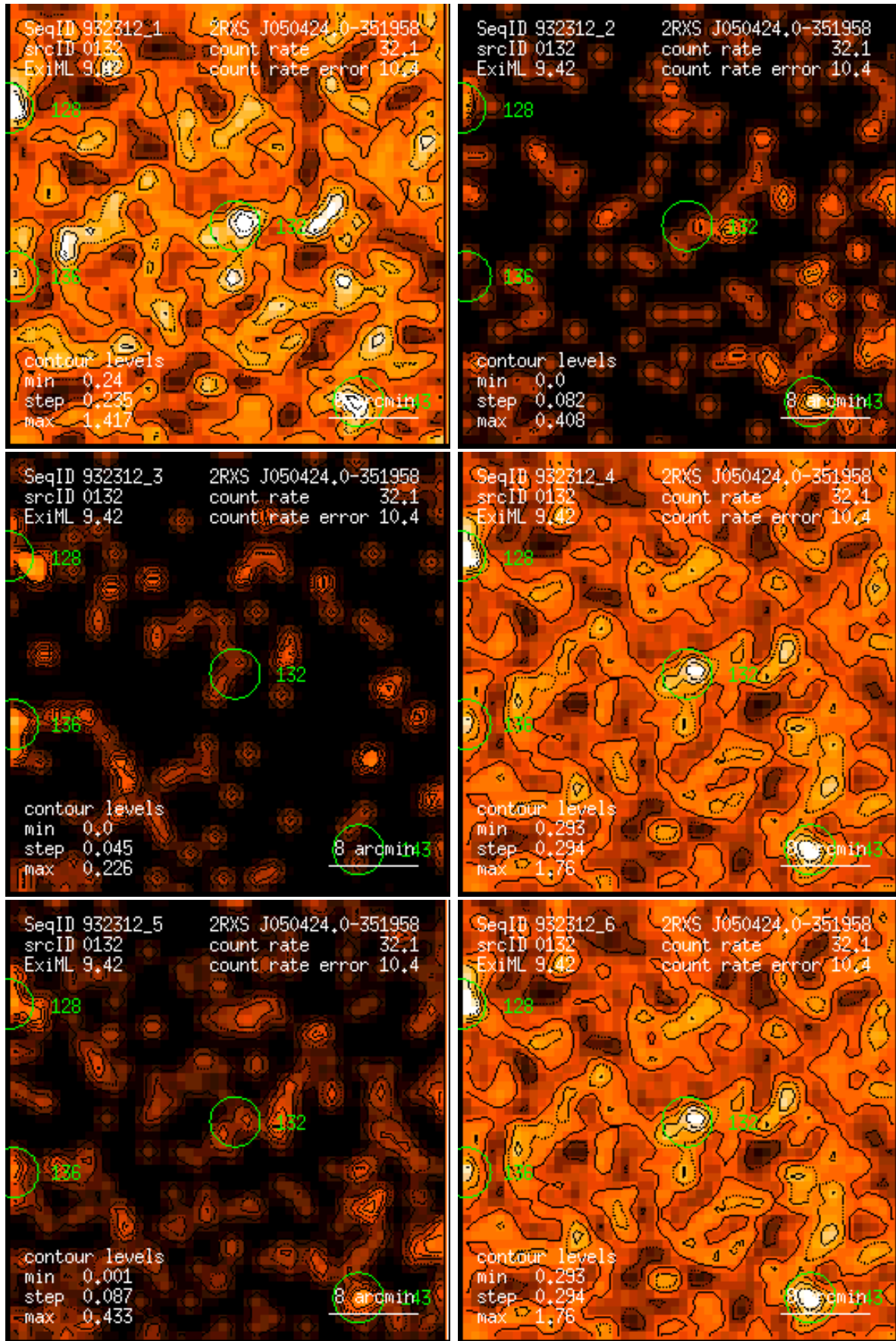
Figure 132: RASS 932312: detection 0132: band rate images, Gaussian filter: (1) PSPPC channels 11 – 41, (2) 52 – 90, (3) 91 – 201, (4) 11 – 235, (5) 52 – 201, (6) 11 – 201. Broad band rates in counts/ks. Band rate contour levels in counts/ks/arcmin 2 .
