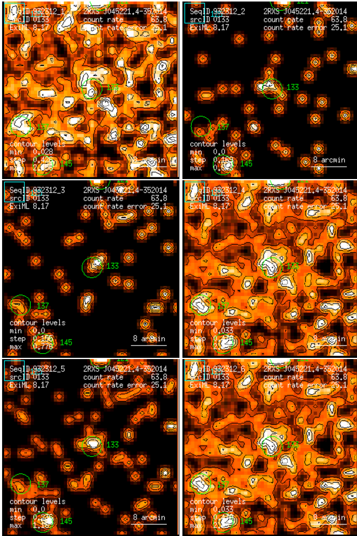
Figure 133: RASS 932312: detection 0133: band rate images, Gaussian filter: (1) PSPC channels 11 – 41, (2) 52 – 90, (3) 91 – 201, (4) 11 – 235, (5) 52 – 201, (6) 11 – 201. Broad band rates in counts/ks. Band rate contour levels in counts/ks/arcmin 2 .
