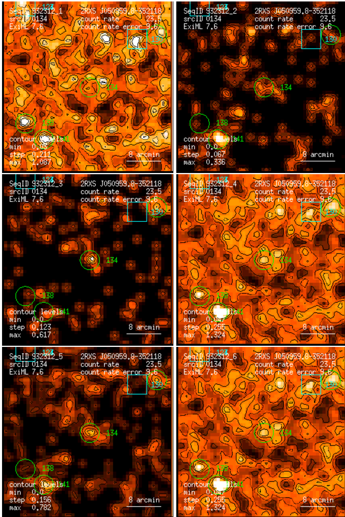
Figure 134: RASS 932312: detection 0134: band rate images, Gaussian filter: (1) PSPC channels 11 – 41, (2) 52 – 90, (3) 91 – 201, (4) 11 – 235, (5) 52 – 201, (6) 11 – 201. Broad band rates in counts/ks. Band rate contour levels in counts/ks/arcmin 2 .
