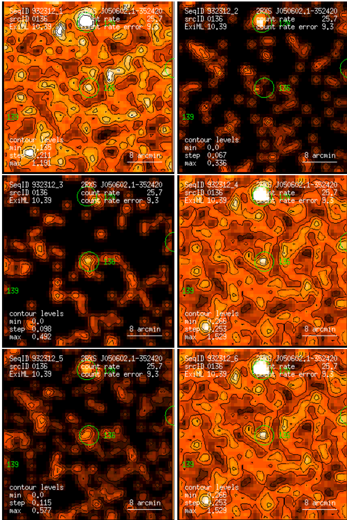
Figure 136: RASS 932312: detection 0136: band rate images, Gaussian filter: (1) PSPC channels 11 – 41, (2) 52 – 90, (3) 91 – 201, (4) 11 – 235, (5) 52 – 201, (6) 11 – 201. Broad band rates in counts/ks. Band rate contour levels in counts/ks/arcmin 2 .
