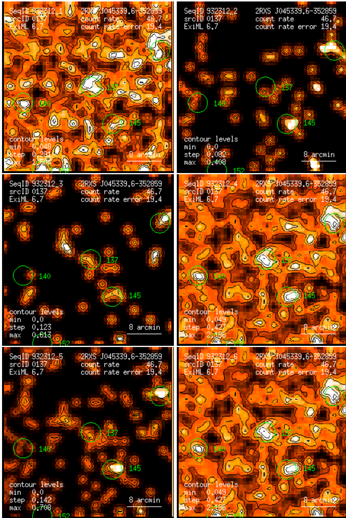
Figure 137: RASS 932312: detection 0137: band rate images, Gaussian filter: (1) PSPC channels 11 – 41, (2) 52 – 90, (3) 91 – 201, (4) 11 – 235, (5) 52 – 201, (6) 11 – 201. Broad band rates in counts/ks. Band rate contour levels in counts/ks/arcmin 2 .
