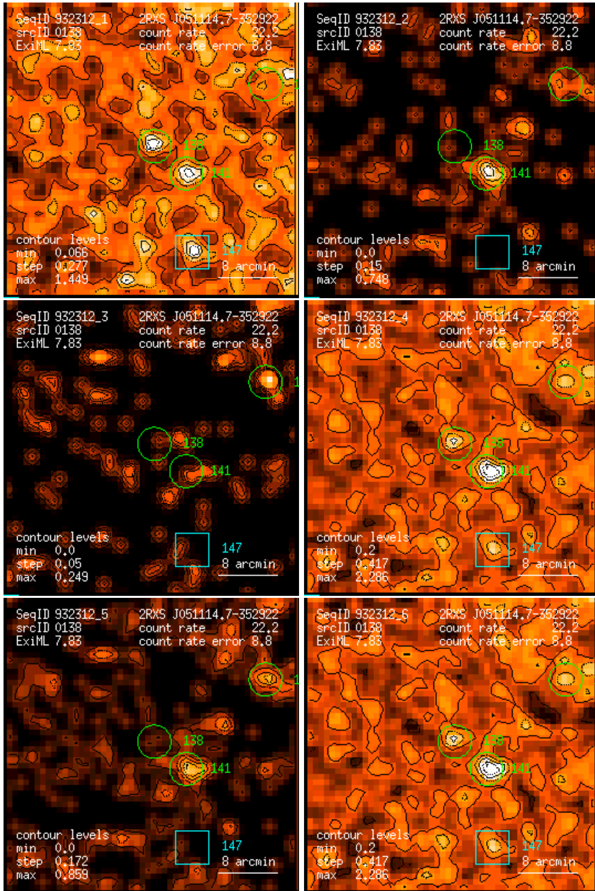
Figure 138: RASS 932312: detection 0138: band rate images, Gaussian filter: (1) PSPC channels 11 – 41, (2) 52 – 90, (3) 91 – 201, (4) 11 – 235, (5) 52 – 201, (6) 11 – 201. Broad band rates in counts/ks. Band rate contour levels in counts/ks/arcmin 2 .
