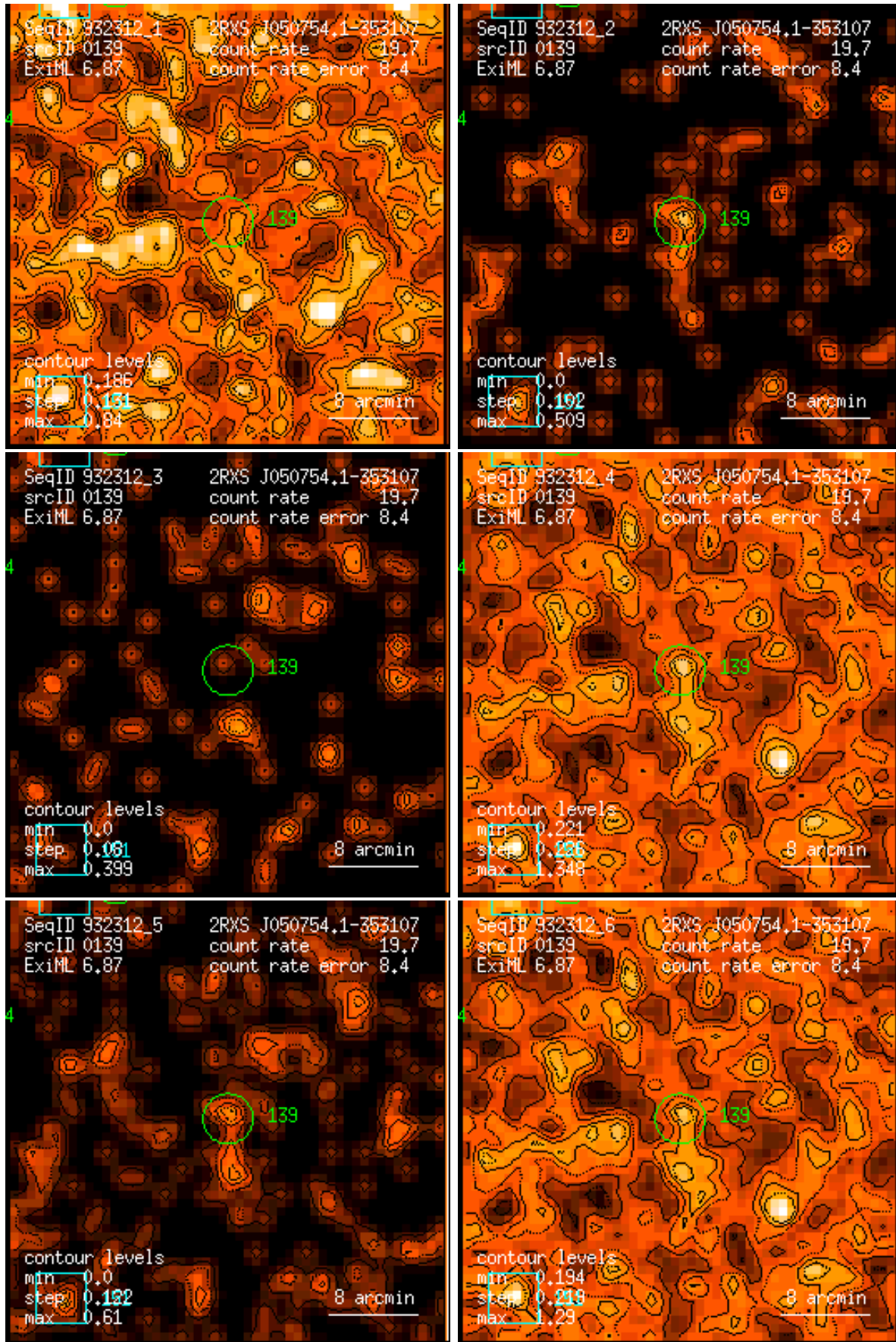
Figure 139: RASS 932312: detection 0139: band rate images, Gaussian filter: (1) PSPC channels 11 – 41, (2) 52 – 90, (3) 91 – 201, (4) 11 – 235, (5) 52 – 201, (6) 11 – 201. Broad band rates in counts/ks. Band rate contour levels in counts/ks/arcmin 2 .
