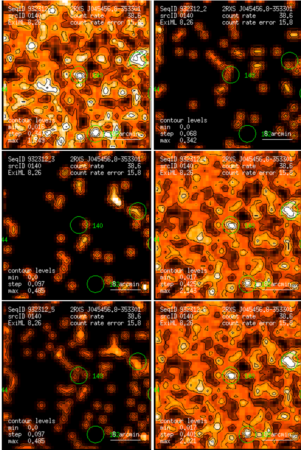
Figure 140: RASS 932312: detection 0140: band rate images, Gaussian filter: (1) PSPC channels 11 – 41, (2) 52 – 90, (3) 91 – 201, (4) 11 – 235, (5) 52 – 201, (6) 11 – 201. Broad band rates in counts/ks. Band rate contour levels in counts/ks/arcmin 2 .
