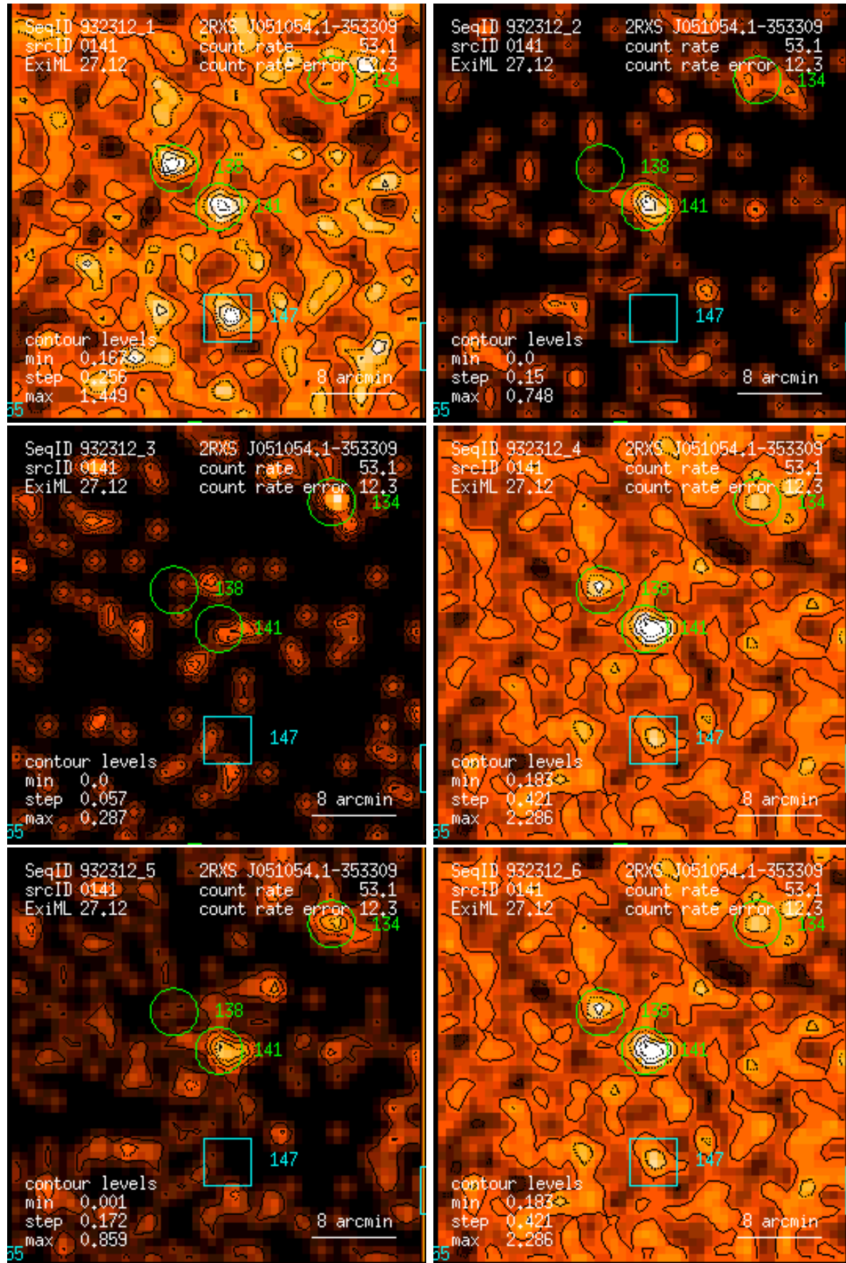
Figure 141: RASS 932312: detection 0141: band rate images, Gaussian filter: (1) PSPC channels 11 – 41, (2) 52 – 90, (3) 91 – 201, (4) 11 – 235, (5) 52 – 201, (6) 11 – 201. Broad band rates in counts/ks. Band rate contour levels in counts/ks/arcmin 2 .
