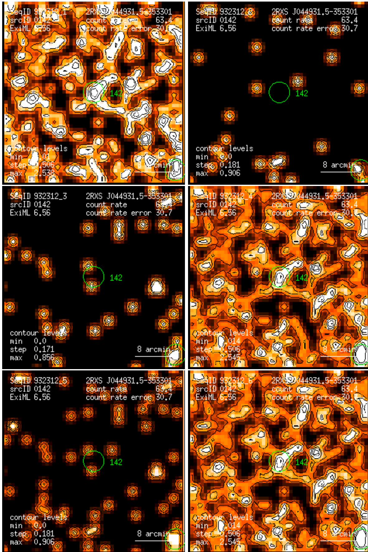
Figure 142: RASS 932312: detection 0142: band rate images, Gaussian filter: (1) PSPC channels 11 – 41, (2) 52 – 90, (3) 91 – 201, (4) 11 – 235, (5) 52 – 201, (6) 11 – 201. Broad band rates in counts/ks. Band rate contour levels in counts/ks/arcmin 2 .
