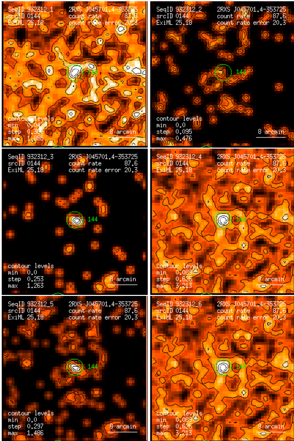
Figure 144: RASS 932312: detection 0144: band rate images, Gaussian filter: (1) PSPC channels 11 – 41, (2) 52 – 90, (3) 91 – 201, (4) 11 – 235, (5) 52 – 201, (6) 11 – 201. Broad band rates in counts/ks. Band rate contour levels in counts/ks/arcmin 2 .
