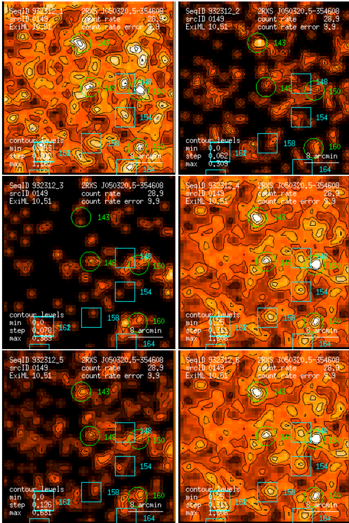
Figure 149: RASS 932312: detection 0149: band rate images, Gaussian filter: (1) PSPC channels 11 – 41, (2) 52 – 90, (3) 91 – 201, (4) 11 – 235, (5) 52 – 201, (6) 11 – 201. Broad band rates in counts/ks. Band rate contour levels in counts/ks/arcmin 2 .
