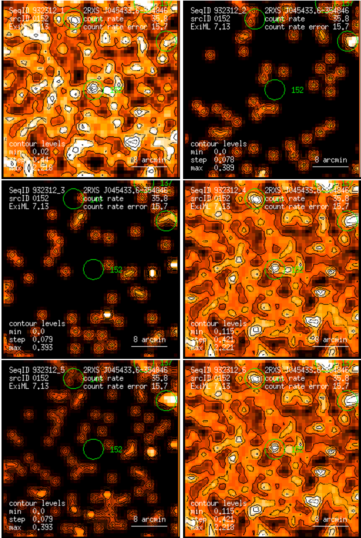
Figure 152: RASS 932312: detection 0152: band rate images, Gaussian filter: (1) PSPC channels 11 – 41, (2) 52 – 90, (3) 91 – 201, (4) 11 – 235, (5) 52 – 201, (6) 11 – 201. Broad band rates in counts/ks. Band rate contour levels in counts/ks/arcmin 2 .
