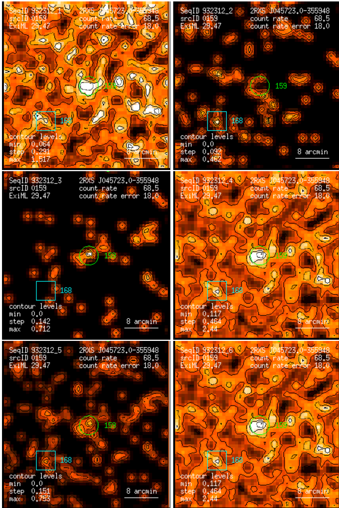
Figure 159: RASS 932312: detection 0159: band rate images, Gaussian filter: (1) PSPC channels 11 – 41, (2) 52 – 90, (3) 91 – 201, (4) 11 – 235, (5) 52 – 201, (6) 11 – 201. Broad band rates in counts/ks. Band rate contour levels in counts/ks/arcmin 2 .
