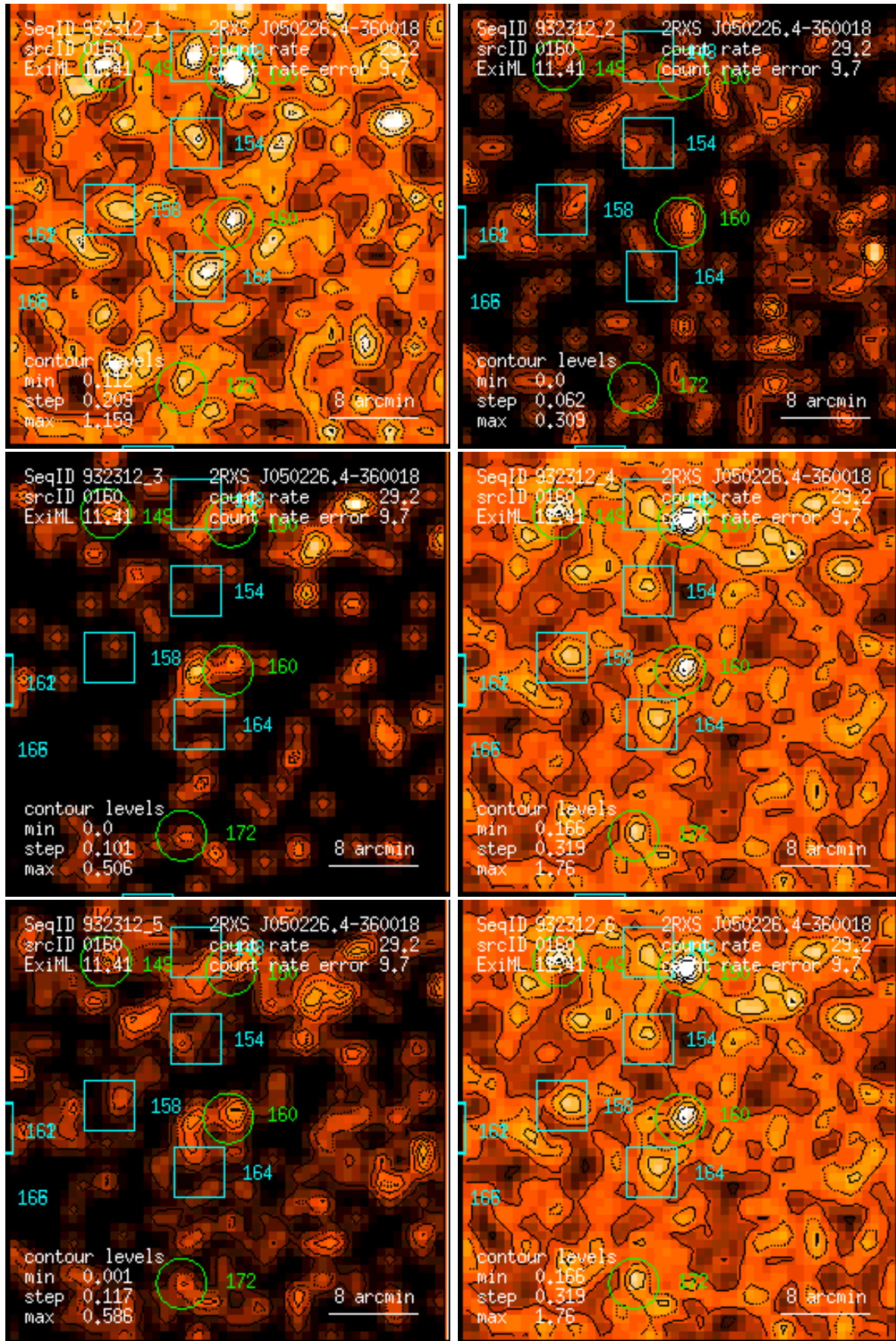
Figure 160: RASS 932312: detection 0160: band rate images, Gaussian filter: (1) PSPC channels 11 – 41, (2) 52 – 90, (3) 91 – 201, (4) 11 – 235, (5) 52 – 201, (6) 11 – 201. Broad band rates in counts/ks. Band rate contour levels in counts/ks/arcmin 2 .
