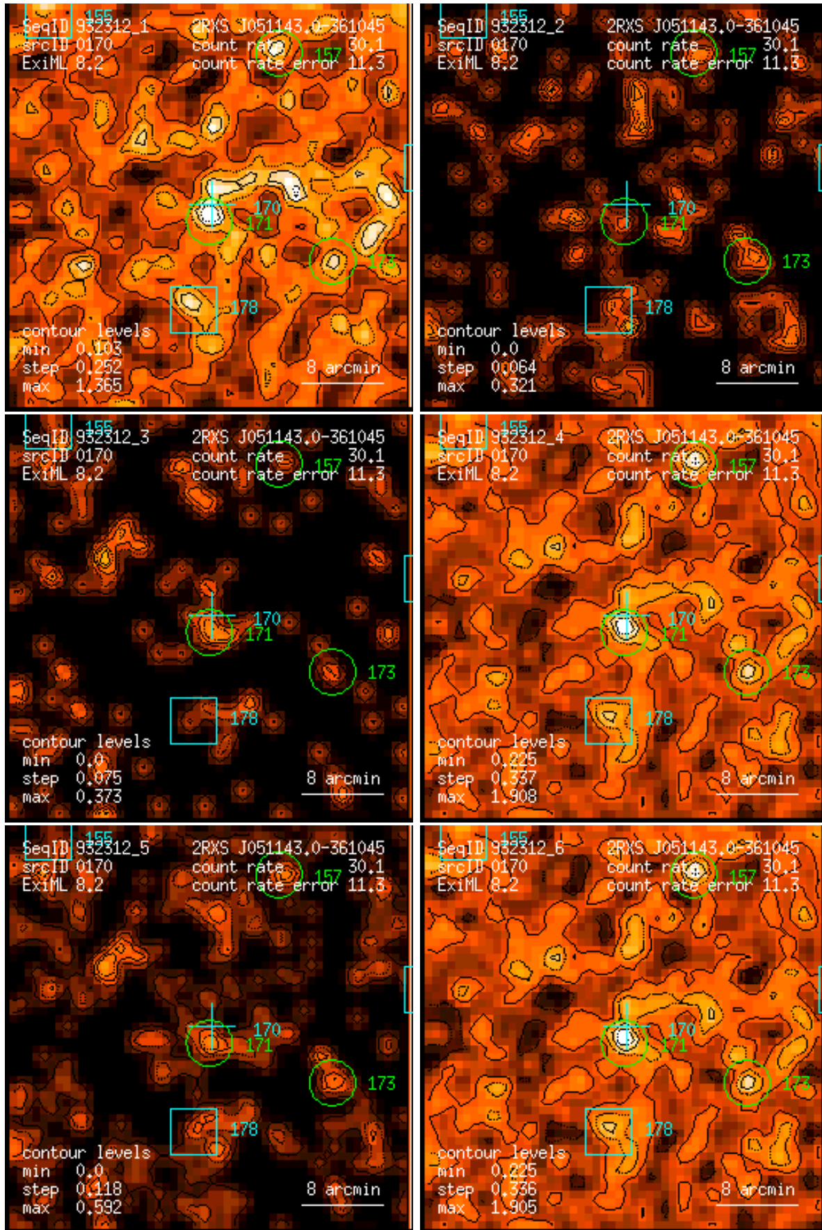
Figure 170: RASS 932312: detection 0170: band rate images, Gaussian filter: (1) PSPC channels 11 – 41, (2) 52 – 90, (3) 91 – 201, (4) 11 – 235, (5) 52 – 201, (6) 11 – 201. Broad band rates in counts/ks. Band rate contour levels in counts/ks/arcmin 2 .
