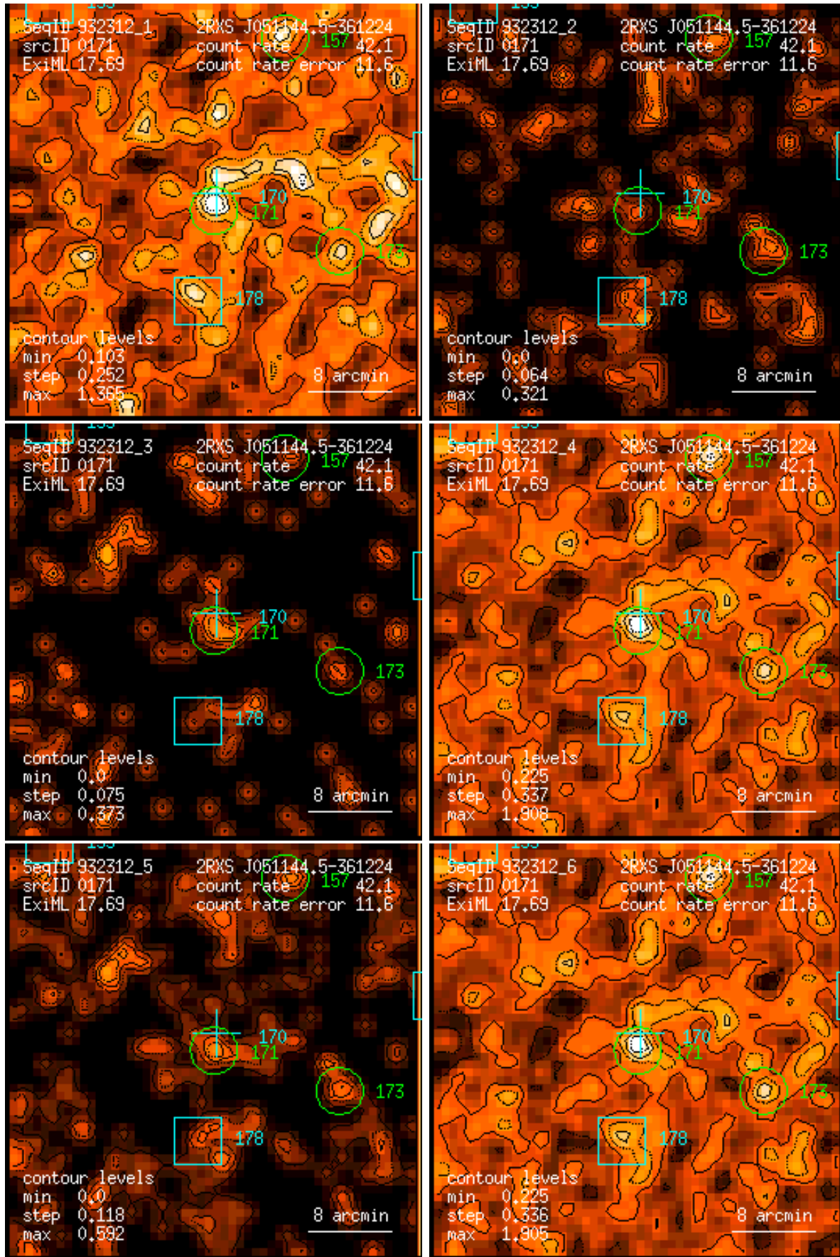
Figure 171: RASS 932312: detection 0171: band rate images, Gaussian filter: (1) PSPC channels 11 – 41, (2) 52 – 90, (3) 91 – 201, (4) 11 – 235, (5) 52 – 201, (6) 11 – 201. Broad band rates in counts/ks. Band rate contour levels in counts/ks/arcmin 2 .
