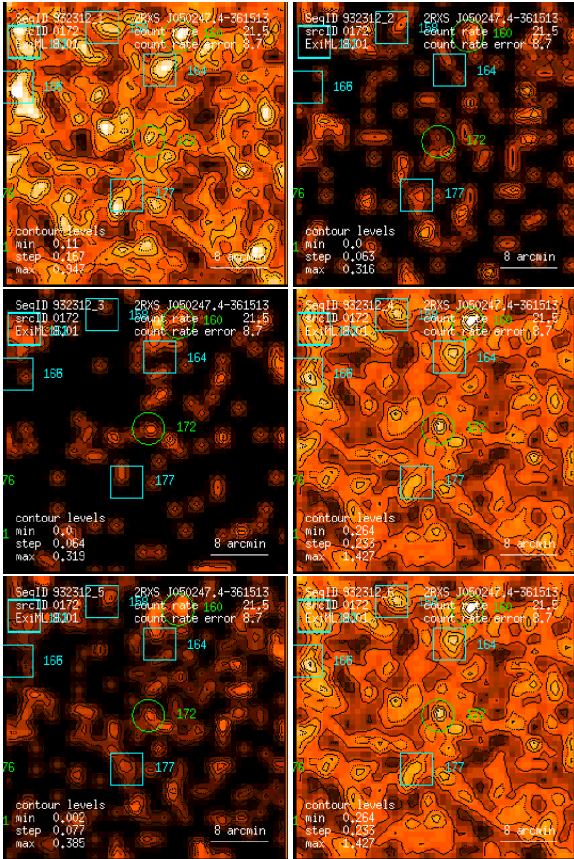
Figure 172: RASS 932312: detection 0172: band rate images, Gaussian filter: (1) PSPC channels 11 – 41, (2) 52 – 90, (3) 91 – 201, (4) 11 – 235, (5) 52 – 201, (6) 11 – 201. Broad band rates in counts/ks. Band rate contour levels in counts/ks/arcmin 2 .
