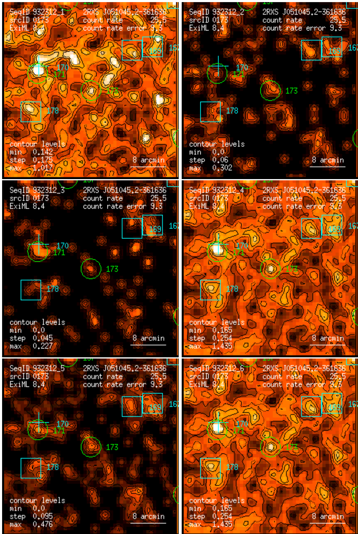
Figure 173: RASS 932312: detection 0173: band rate images, Gaussian filter: (1) PSPC channels 11 – 41, (2) 52 – 90, (3) 91 – 201, (4) 11 – 235, (5) 52 – 201, (6) 11 – 201. Broad band rates in counts/ks. Band rate contour levels in counts/ks/arcmin 2 .
