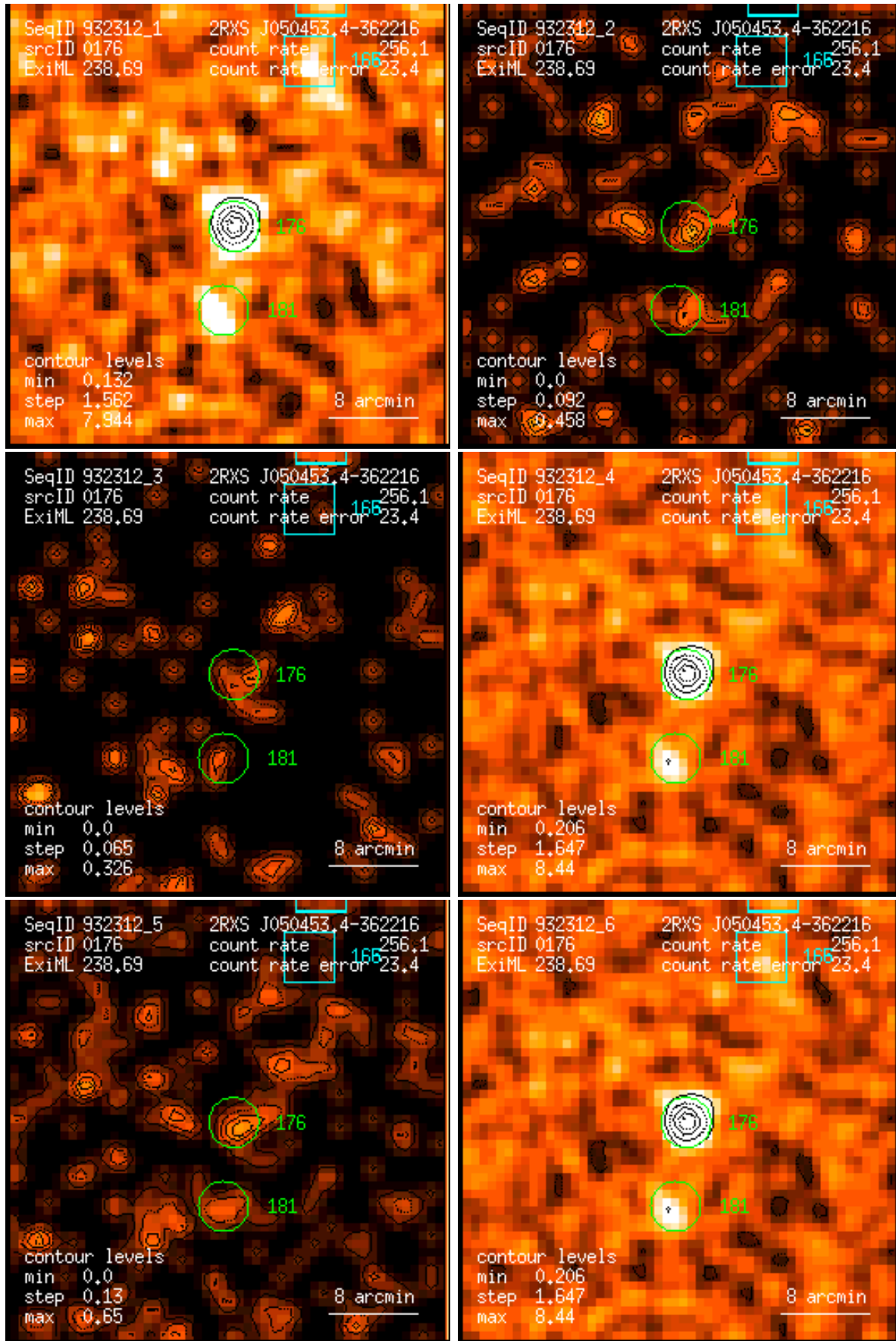
Figure 176: RASS 932312: detection 0176: band rate images, Gaussian filter: (1) PSPC channels 11 – 41, (2) 52 – 90, (3) 91 – 201, (4) 11 – 235, (5) 52 – 201, (6) 11 – 201. Broad band rates in counts/ks. Band rate contour levels in counts/ks/arcmin 2 .
