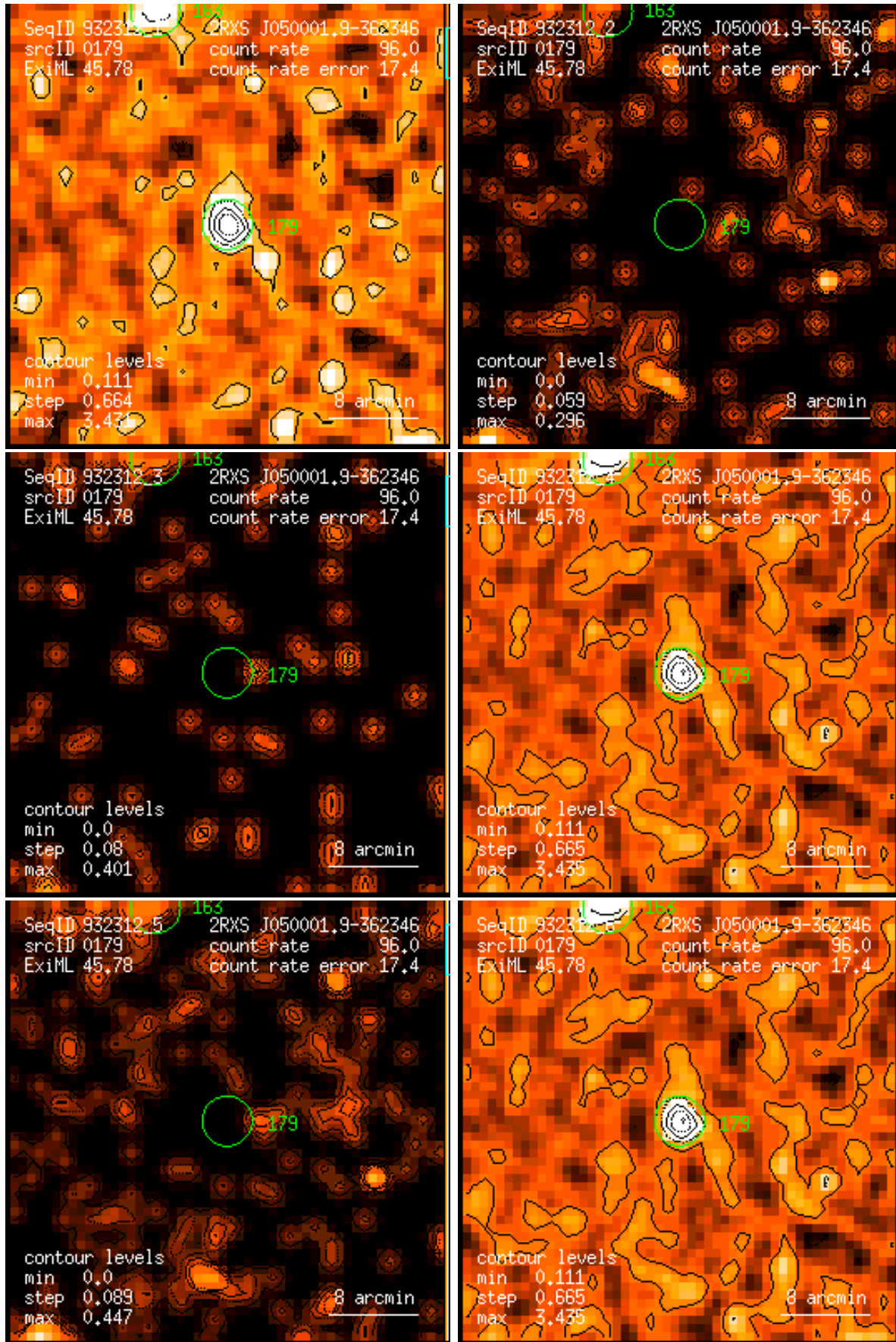
Figure 179: RASS 932312: detection 0179: band rate images, Gaussian filter: (1) PSPC channels 11 – 41, (2) 52 – 90, (3) 91 – 201, (4) 11 – 235, (5) 52 – 201, (6) 11 – 201. Broad band rates in counts/ks. Band rate contour levels in counts/ks/arcmin 2 .
