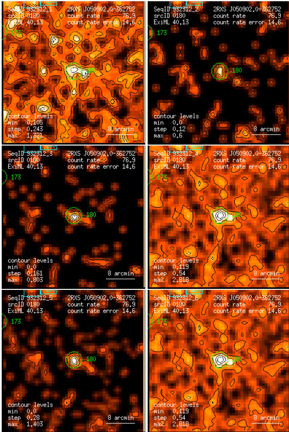
Figure 180: RASS 932312: detection 0180: band rate images, Gaussian filter: (1) PSPC channels 11 – 41, (2) 52 – 90, (3) 91 – 201, (4) 11 – 235, (5) 52 – 201, (6) 11 – 201. Broad band rates in counts/ks. Band rate contour levels in counts/ks/arcmin 2 .
