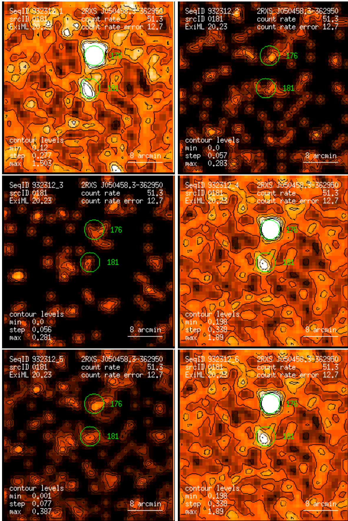
Figure 181: RASS 932312: detection 0181: band rate images, Gaussian filter: (1) PSPC channels 11 – 41, (2) 52 – 90, (3) 91 – 201, (4) 11 – 235, (5) 52 – 201, (6) 11 – 201. Broad band rates in counts/ks. Band rate contour levels in counts/ks/arcmin 2 .
