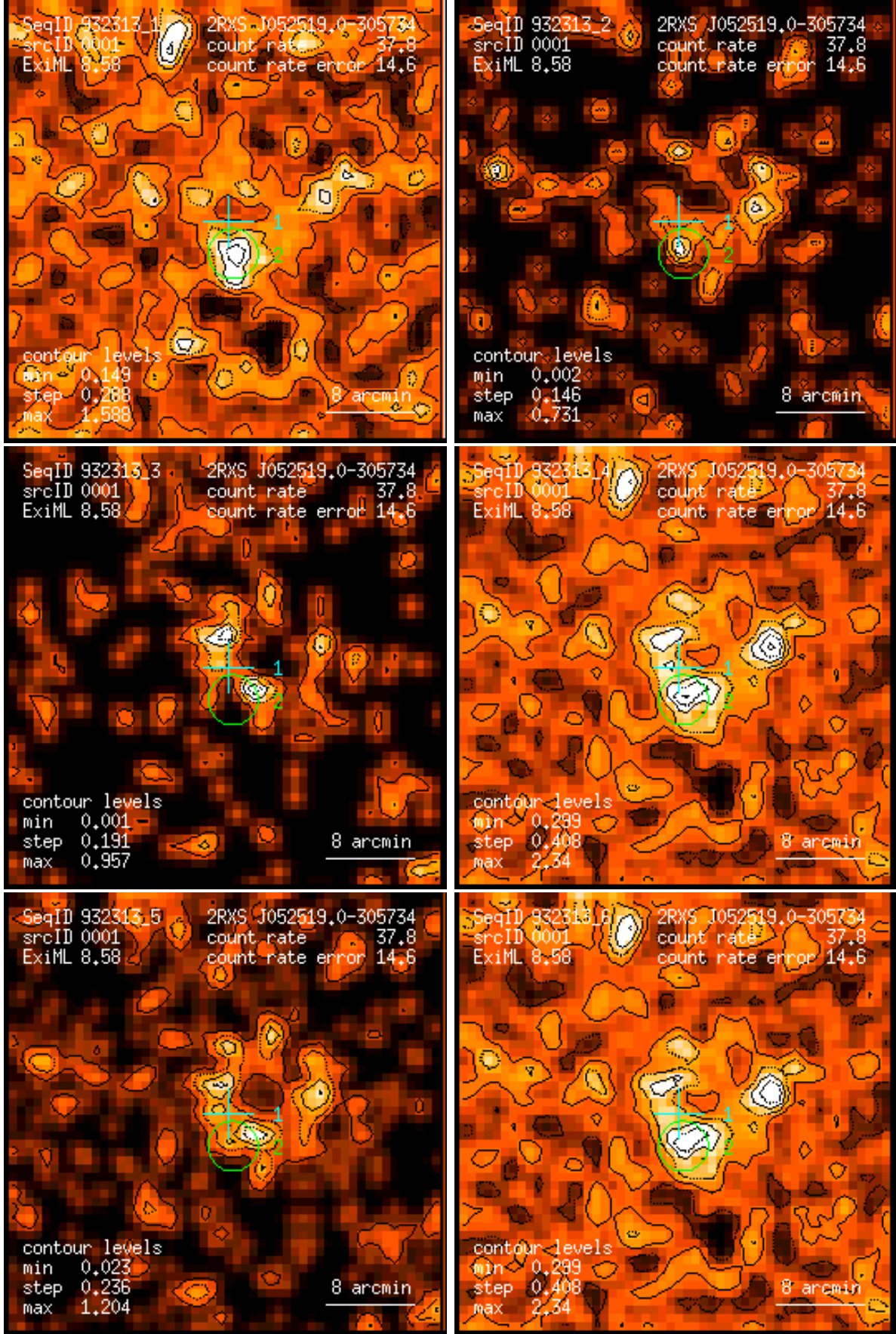
Figure 1: RASS 932313: detection 0001: band rate images, Gaussian filter: (1) PSPC channels 11 – 41, (2) 52 – 90, (3) 91 – 201, (4) 11 – 235, (5) 52 – 201, (6) 11 – 201. Broad band rates in counts/ks. Band rate contour levels in counts/ks/arcmin 2 .
