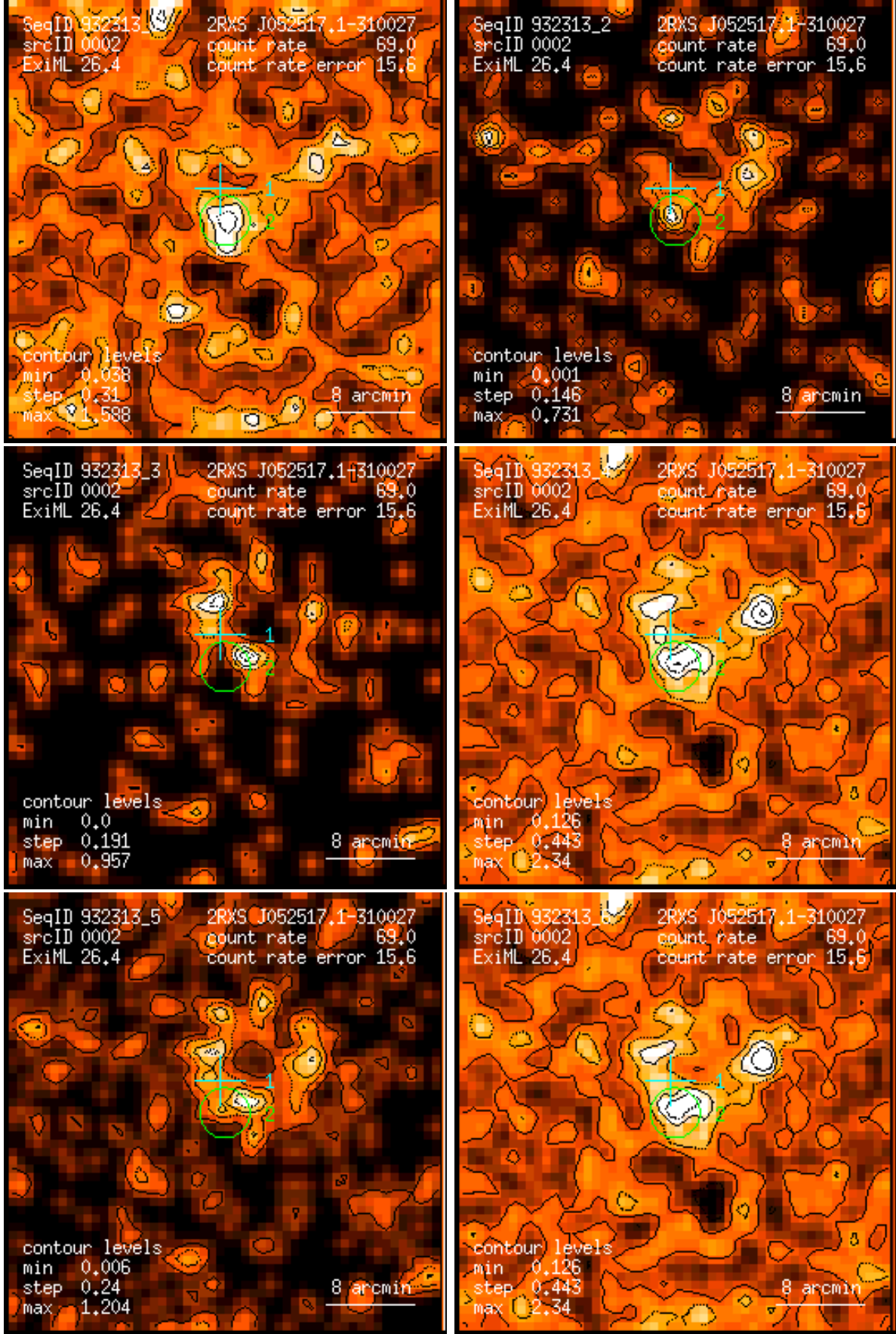
Figure 2: RASS 932313: detection 0002: band rate images, Gaussian filter: (1) PSPC channels 11 – 41, (2) 52 – 90, (3) 91 – 201, (4) 11 – 235, (5) 52 – 201, (6) 11 – 201. Broad band rates in counts/ks. Band rate contour levels in counts/ks/arcmin 2 .
